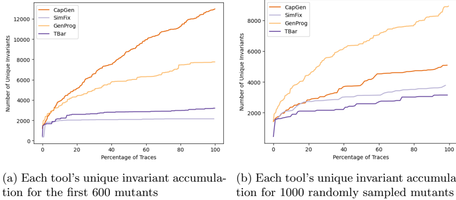
Fig. 2: Unique invariants from each APR tool for Math 80 over time. x -axis is % of traces evaluated, y -axis is the number of unique invariants. Tools that explore more of the search space also find more unique functionality over time.
