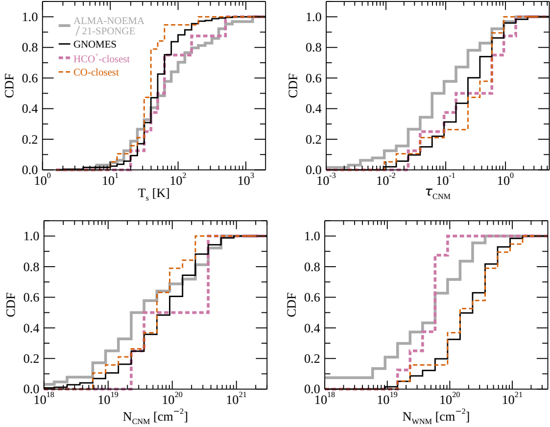
Figure B2. CDFs of the spin temperature, optical depth, CNM and WNM column density. All H I components toward LOSs at b < -5^\circ from the GNOMES and ALMA-NOEMA/21-SPONGE surveys are shown in thin black and thick gray (solid lines). Among these components, those in close proximity to CO and HCO + in velocity are selected and presented in thin tan and thick pink (dashed lines).
