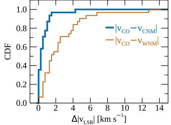
Figure 5. CDF of the absolute velocity difference between H\text{ I} and CO (CNM and CO in thick blue; WNM and CO in thin tan). For these CDFs, H\text{ I} components that are closest to the observed CO emission in velocity were considered.
