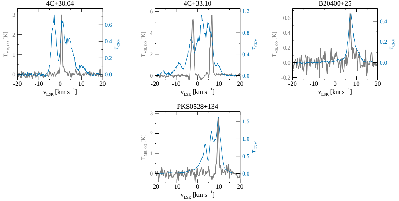
Figure A1. Comparison between the H I absorption (thin blue) and CO emission (thick gray) spectra toward the 19 CO-detected LOSs. The spectra are aligned at peaks for ease of comparison.
