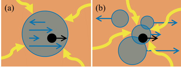
Figure 9. Possible distributions of the WNM, CNM, and CO (tan, blue, and black, respectively). Based on our finding of the kinematic association between H I and CO (Section 6.1), the WNM is represented as the diffuse background, while the CNM and CO are shown as the smaller embedded structures. The velocities of the CNM and CO are indicated as the blue and black arrows with arbitrary sizes, and UV radiation is presented as the yellow arrows. (Left) Scenario for the Entire LOS, where CNM components at different velocities belong to one large structure and contribute to the shielding of the CO core. (Right) Scenario for Cases A and B, where CNM components close to CO only provide shielding against UV radiation.
