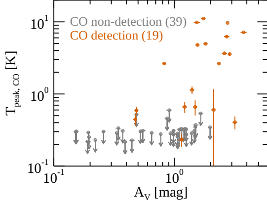
Figure 8. CO peak brightness temperature as a function of Planck -based A_V . The 19 CO-detected LOSs are shown in tan, while upper limits based on 3\sigma values are indicated as the downward arrows for the 39 CO non-detected LOSs.
