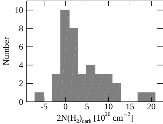
Figure 4. Histogram of the CO-dark H_2 column density for the 39 CO non-detected LOSs.
