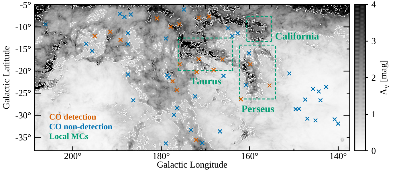
Figure 1. GNOMES LOSs at b < -5^\circ overlaid on the Planck A_V image (Section 4.1; 1, 3, and 5 mag as the white contours). Among the total 58 LOSs, 19 LOSs where CO(1–0) emission is clearly detected are shown as the tan crosses. The remaining 39 LOSs without CO detection are indicated as the blue crosses. The green boxes represent the approximate extents of local molecular clouds (top to bottom: California, Taurus, and Perseus; Lee et al. 2018).
