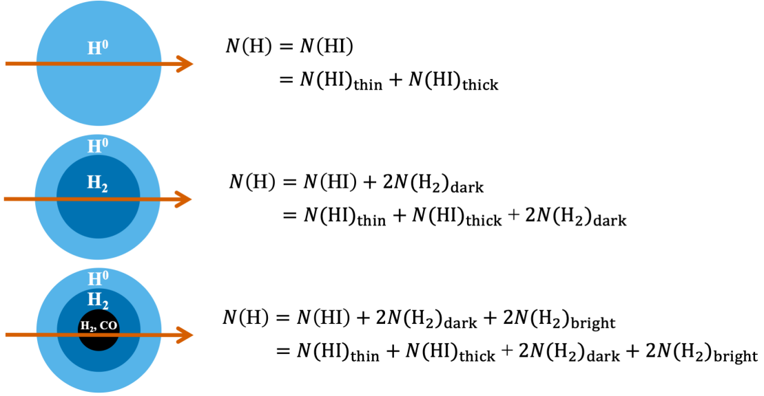
Figure 2. Illustration of LOSs with different gas phases. (Top) H I-only LOSs. (Middle) LOSs with H I and CO-dark H_2 gas. (Bottom) LOSs with H I, CO-dark H_2 , and CO-bright H_2 gas.
