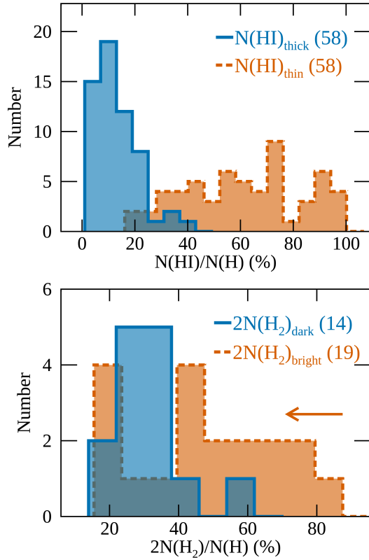
Figure 3. Fraction of each gas phase with respect to the total hydrogen. (Top) Optically thick and thin H I in solid blue and dashed tan. (Bottom) CO-dark and CO-bright H_2 in solid blue and dashed tan. The leftward arrow indicates that the derived fractions for CO-bright H_2 are upper limits.
