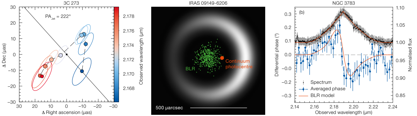
Figure 1. Left: Observed velocity-resolved photocentres for 3C 273 indicating a kinematic axis nearly perpendicular to the radio jet axis (black line) (GRAVITY Collaboration et al., 2018). Middle: Cartoon illustrating a possible cause of the observed offset between the near-infrared continuum photocentre and the
