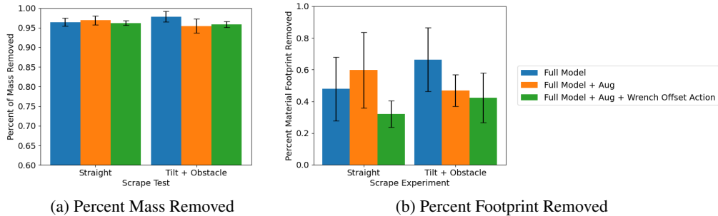
Figure 7: Target Scraping Results: Our ‘Full Model’ and variations for addressing visual occlusions and reaction forces arising from contact with the target object perform comparably on both metrics over 5 trials on each experiment.
