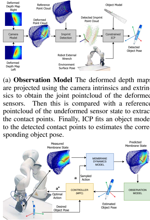
(b) Control Pipeline Given a measured state, our controller queries the membrane dynamics model with sampled actions to obtain the predicted membrane states. The object pose is estimated from the predicted membrane states and it is compared with the desired poses to compute the costs associated to the sample actions. The costs are aggregated and the resultant optimal action is executed by the robot.
