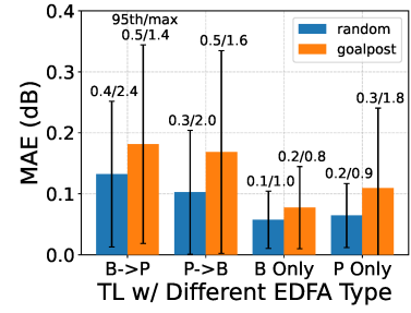
Fig. 6: TL between different EDFA types (B: booster, P: pre-amplifier).
