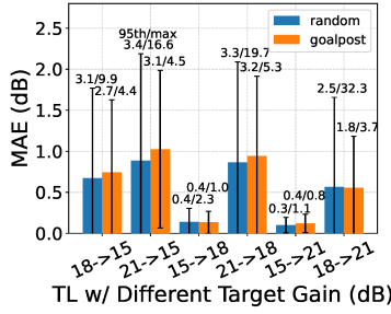
Fig. 5: TL from one source gain setting (left) or two source gain settings (right) to another target gain setting on the same booster EDFA.
