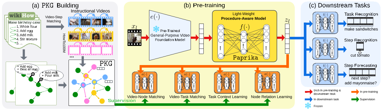
Figure 2. Overview. We encode procedural knowledge in a Procedural Knowledge Graph (PKG): nodes are (clustered) steps from wikiHow that are annotated with features, and edges connect steps that occur sequentially in the instructional activities from wikiHow or an unlabeled instructional video corpus. Four pre-training objectives elicit the knowledge in the PKG to Paprika, a procedure-aware model. We achieve this by querying the PKG to produce pseudo labels for pre-training as supervisory signals. Paprika learns a video representation that encodes procedural knowledge and thus lead to improved performance on multiple downstream procedure understanding tasks.
