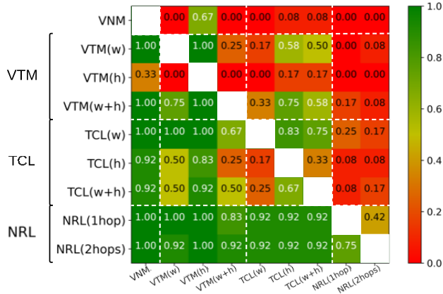
Figure 3. Overall Performance Comparison. This matrix compares the overall performance of our proposed pre-training objectives. The value in entry (i, j) is the ratio of evaluation settings in which the accuracy of method i is greater than the accuracy of method j. Here, 1 indicates method i outperforms method j in all 12 evaluation settings. The more green entries in the row of a method, the better its overall performance. NRL is the most effective method.
