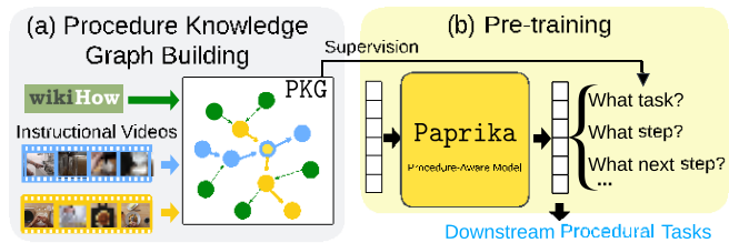
Figure 1. Training a video representation for procedure understanding with supervision from a procedural knowledge graph: the structure observed in instructions for procedures (from text, from videos) corresponds to sequences of steps that repeat between instances of the same or different tasks; this structure is well represented by a Procedural Knowledge Graph (PKG). (a) We build a PKG combining text instructions with unlabeled video data, and (b) obtain a video representation by encoding the human procedural knowledge from the PKG into a more general procedure-aware model ( Paprika ) generating pseudo labels with the PKG for several procedure understanding objectives. Paprika can then be easily applied to multiple downstream procedural tasks.
