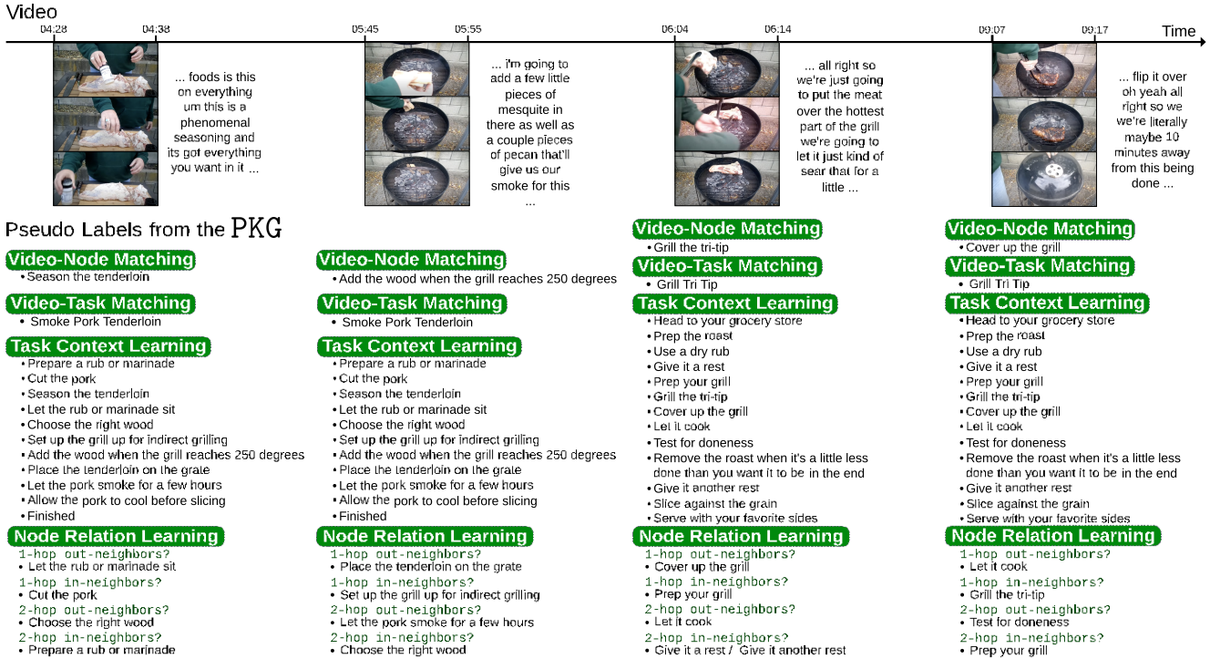
Figure 4. Pseudo labels generated by the PKG of one video (title is “Grilling A Tri-Tip ...”). Frames and temporally overlapped subtitles of four segments sampled from this video were shown. For a succinct visualization, for each pre-training objective, we only show the result of the most confident pseudo label. TCL and NRL provide more procedure-level context information than VNM and VTM. Our pseudo labels entail a much higher relevance to each segment than the subtitle and allow Paprika to leverage cross-task information sharing.
