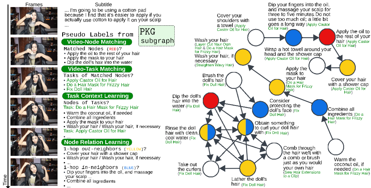
Figure 5. Pseudo labels of one segment and the subgraph of the PKG that this segment belongs to. The PKG encodes the procedural knowledge of the general order and relation of steps from multiple tasks. This is because a node’s k-hop neighbors can come from multiple tasks, and the edge direction encodes the general execution order of steps (the order that was observed in data – not in one specific video).
