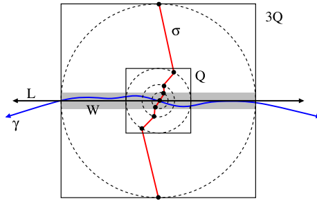
Fig. 6. If all the \beta 's are small at p , and p is a tangent point of \gamma , then \gamma must cross Q in the sense that the orthogonal projection of \gamma \cap 3Q on the line L must cover L \cap Q , i.e., \gamma can't "double back" and leave using the same end of W that it entered.
