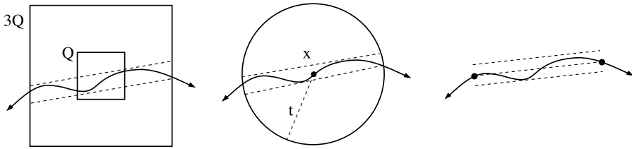
Fig. 8. Three equivalent versions of the \beta -numbers.
