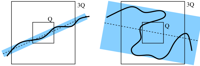
Fig. 1. The definition of the \beta -numbers. The left shows a situation where \beta_E(Q) is small and the right a situation where it is large. The shaded region represents the thinnest strip containing E \cap 3Q and the dashed line is its axis, the line L in the definition of \beta_E(Q) .
