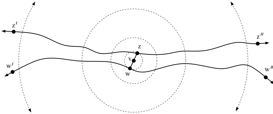
Fig. 7. If \Gamma does not have bounded turning, then there are points z, w that cannot be connected by a subarc of diameter O(|z - w|) . This means these points lie on disjoint subarcs whose four endpoints are all distance \gg |z - w| from z and w .
