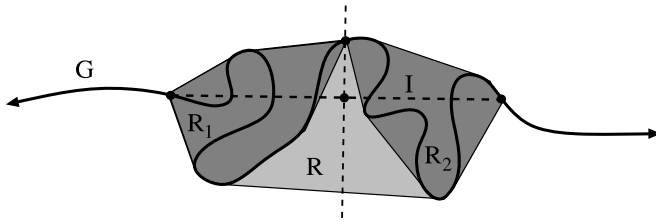
Fig. 2. The convex set R is split into two smaller convex sets.
