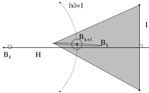
Fig. 3. If the hyperplane H passes very close to the center of a k -dimensional ball B_k that lies on one side of H , then B_k is nearly parallel to H and a concentric ball of comparable radius and dimension k + 1 lies in the convex hull of B_k and any segment I that is bisected and perpendicular to H , and whose length is comparable to its distance from B_k . This implies the common ancestor of two disjoint sets with very close centers must have strictly larger rank than either of them.
