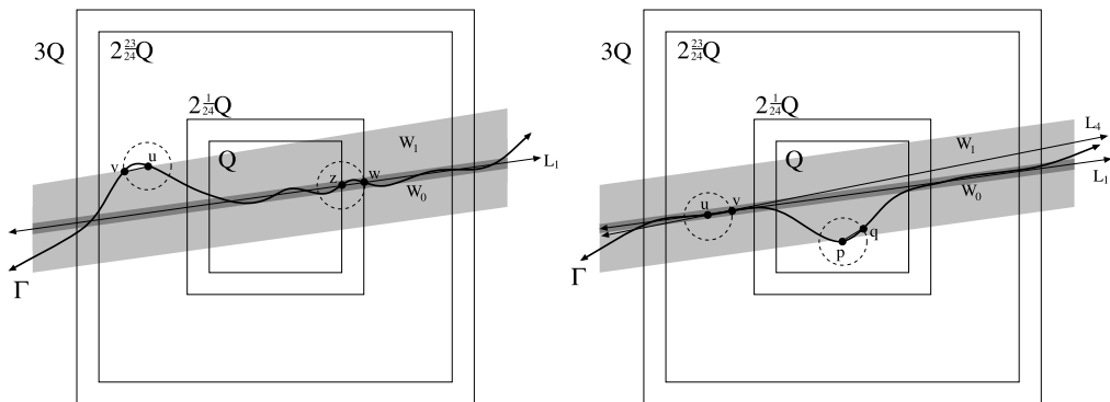
Fig. 4. In both cases, we can find two segments inside 3Q that have lengths comparable to \text{diam}(Q) and are not both close to common line. Lemma 3.3 then implies at least measure \simeq \beta^2 of hyperplanes hit both segments. For clarity, the pictures are not quite to scale.
