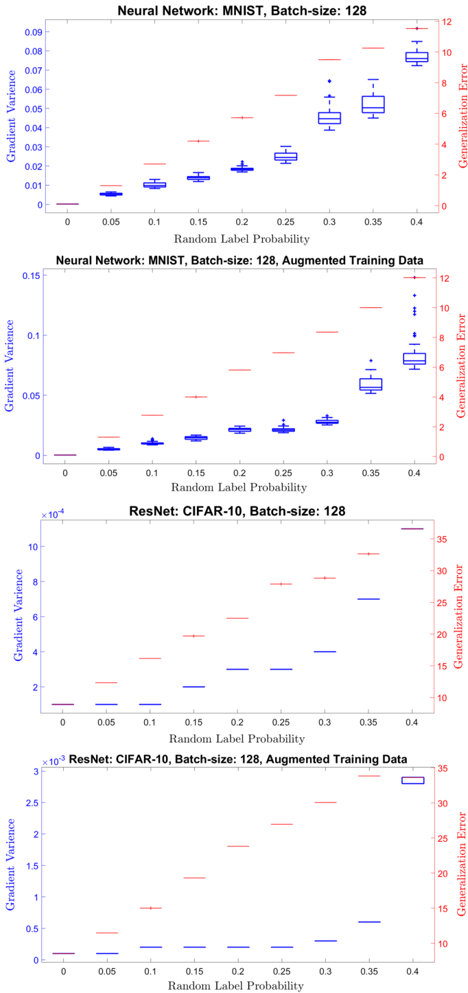
Fig. 3 Comparison of on-average variance, generalization error and random label probability with/without data augmentation
