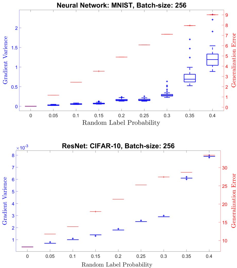
Fig. 1 Relation of on-average variance (left y axis), generalization error (right y axis) and random label probability (x axis) in training MLP and ResNet using SGD
