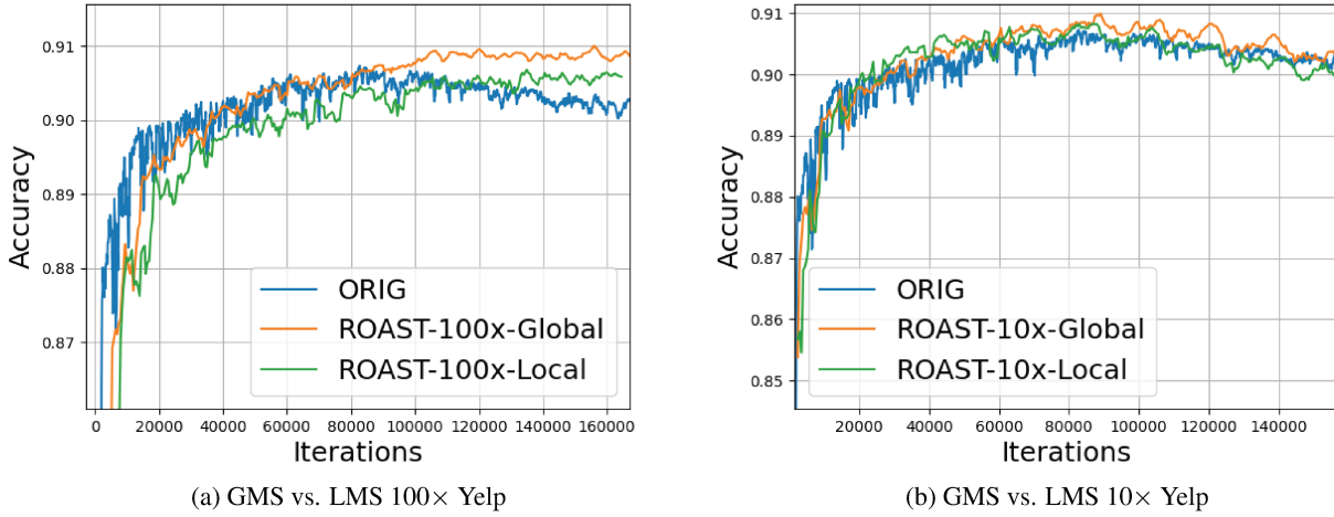
Figure 3. Separate plots for 10× and 100× ROAST for Yelp dataset for better visibility. Also, rolling mean of 5 measurements was used to reduce noise in the plots
