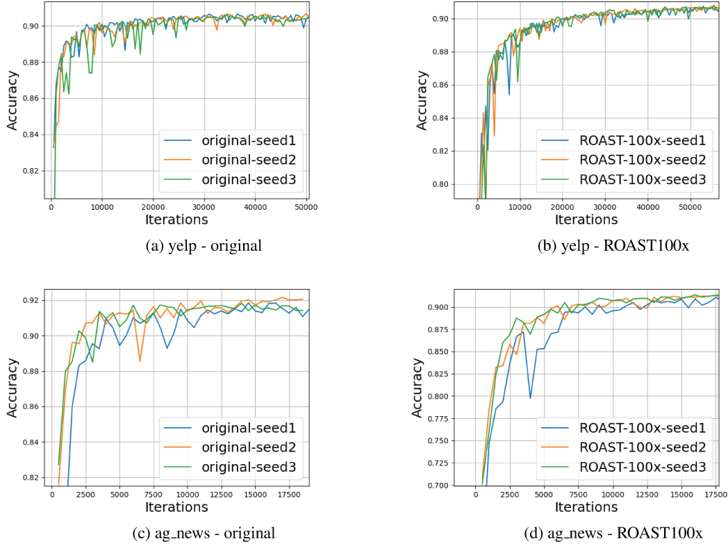
Figure 4. Three runs of original and ROAST-100x runs
