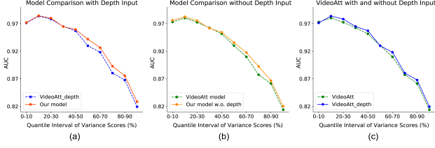
Figure 7: Comparison of AUC in each quantile interval in the GazeFollow test set. Our model shows obviously higher AUC in intervals with larger annotation variance, which cannot be observed in (c) when adding depth input only.
