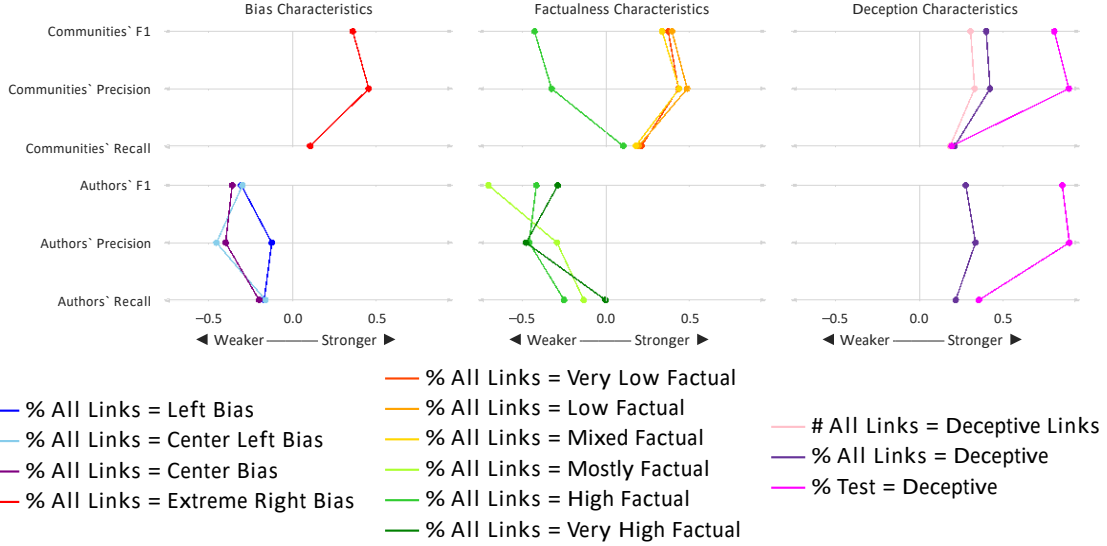
Figure 4: Correlation coefficients between characteristics and aggregated community/author performance metrics: F1, precision, and recall. All characteristics with an absolute Pearson’s r correlation coefficient greater than 0.3 for at least one metric are included. Generally, stronger model performance is correlated with more right bias, low factual, and deceptive content, while weaker performance is correlated with more left bias and high factual content.
