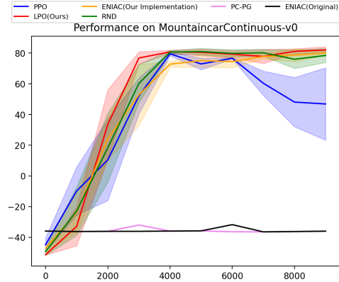
Figure 2. Performance comparison between the original implementations of ENIAC , PC-PG and our implementation of ENIAC , LPO . Lines are evaluation results averaged over 5 random seeds every 10k steps, the shaded area represents the standard deviation.
