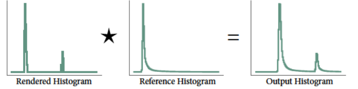
Fig. 2: The raw rendered histogram is cross-correlated with the reference histogram (which encodes the laser pulse intensity over time) to generate the output histogram of our forward imaging model.
