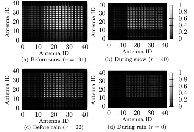
Figure 8: Impact of Snow and Rain on Low-UHF mMIMO Channel Correlation
