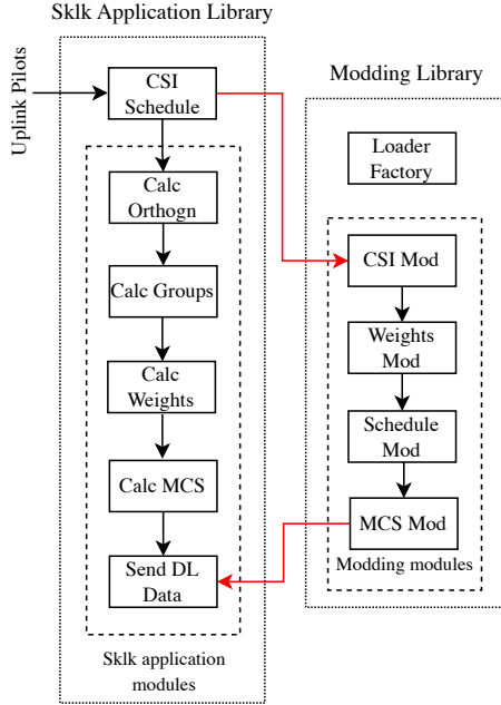
Figure 5: Modding API Architecture
