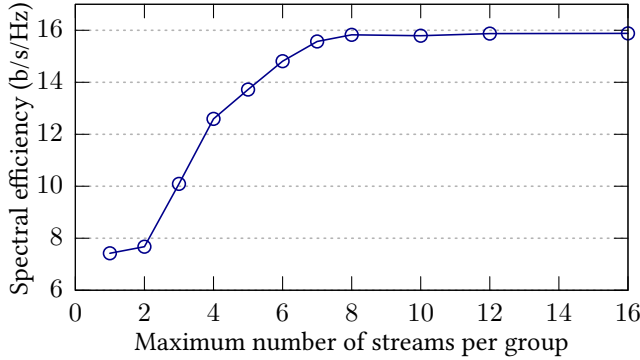
Figure 14: Impact of Increasing Spatial Streams on Spectral Efficiency
