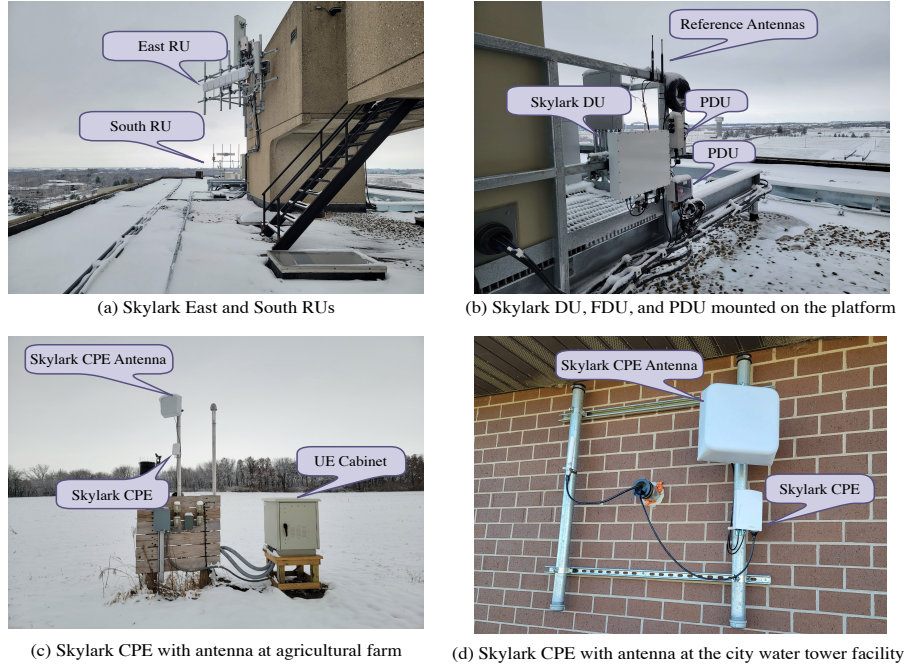
Figure 3: Field Deployment of Skylark Faros V2 System
