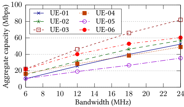
Figure 10: Aggregate Capacity (UL + DL) for Each UE
