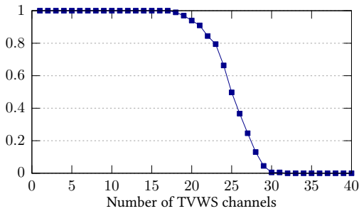
Figure 2: CCDF of Available TVWS Channels in AraMIMO
