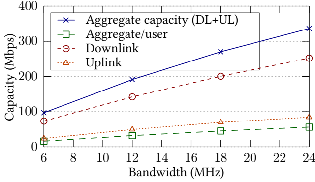
Figure 9: DL, UL, and Aggregate capacity for 6 UEs
