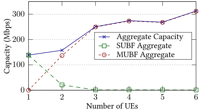
Figure 12: Impact of Number of UEs on System Capacity
