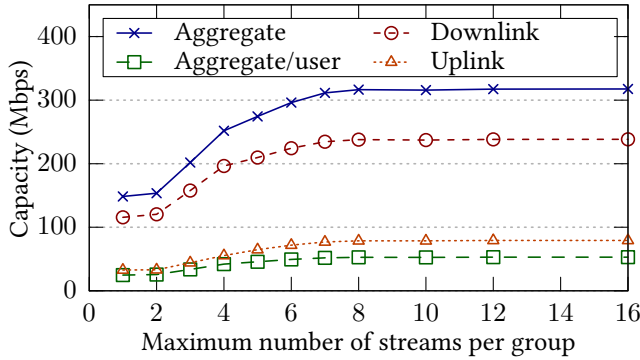
Figure 13: Impact of Maximum Number of Streams on System Capacity
