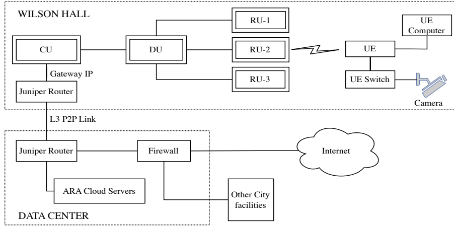
Figure 4: Skylark Deployment Architecture
