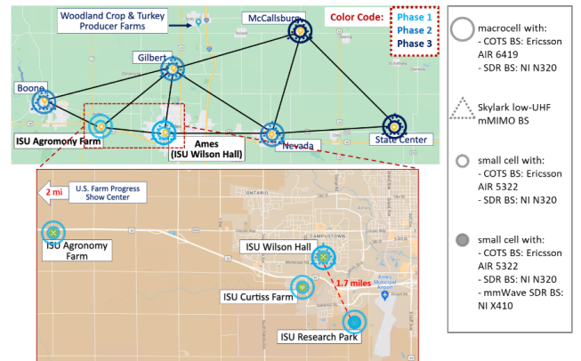
Figure 1: ARA PAWR Deployment
