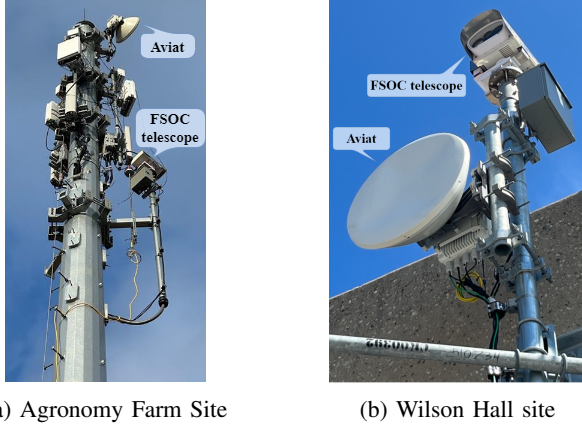
Fig. 2: Aviat dish antennas and FSOC telescopes of AraHaul.
