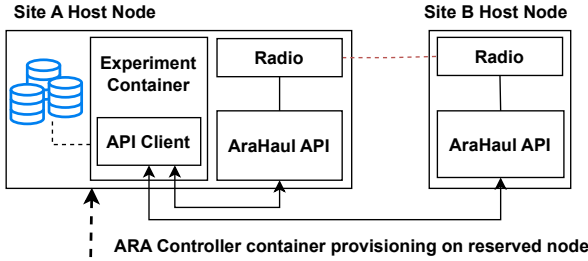
Fig. 4: Software view of the experimental setup.
