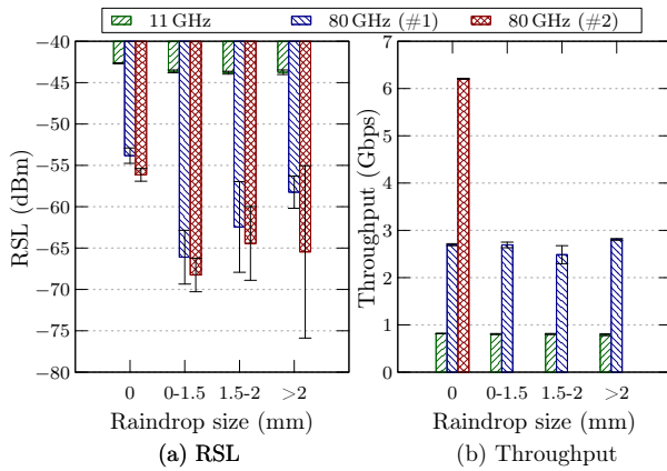
Fig. 7: Impact of raindrop size on AraHaul links (CI=95%).
