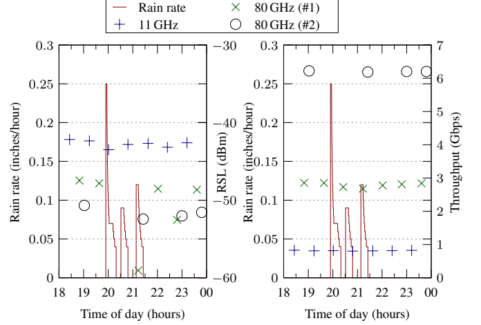
Fig. 5: Behaviors of AraHaul links over a distance of 6.31 miles (or 10.15 km) during a 6-hour time period with varying rain rates. Three groups of results are plotted: 11 GHz ('+' points), 80 GHz Config #1 ('x' points) and Config #2 ('o' points). Details of the configurations are listed in Table V. Rain conditions were reported by the Lufft WS100 disdrometer, RSL data were reported by the Aviat WTM 4811 radio, and link throughput was measured by iPerf.
