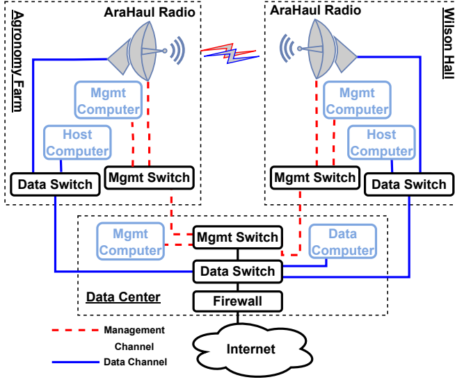
Fig. 3: AraHaul hardware and network architecture.
