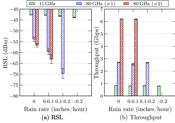
Fig. 6: Impact of rain rate on AraHaul links (CI=95%).
