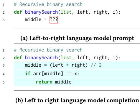
Figure 4: Left-to-right language model code generation
