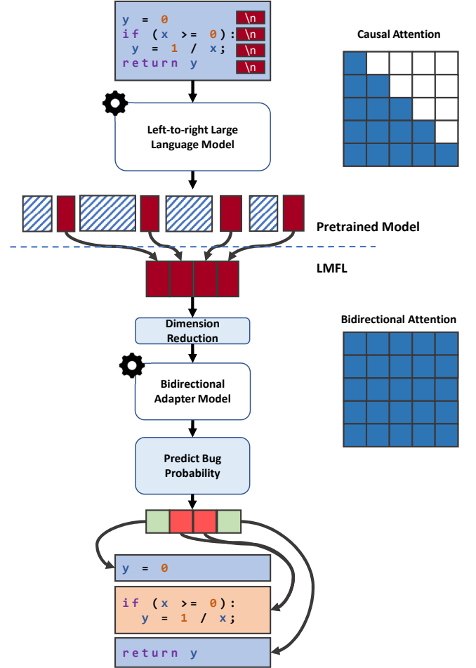
Figure 5: Attention masking procedure of LLMAO
