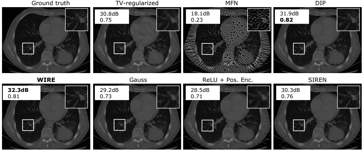
Figure 9. Computed tomography reconstruction. Inverse problems with noisy undersampled data require a strong signal prior for robust reconstruction. Here, we show CT-based reconstruction with 100 angles for a 256 \times 256 image ( 2.5\times compression) with various approaches. WIRE results in sharp reconstruction, exposing features that are blurry, or with ringing artifacts in reconstructions with other approaches. WIRE is hence a strong signal prior for images, and can solve a large class of inverse problems.
