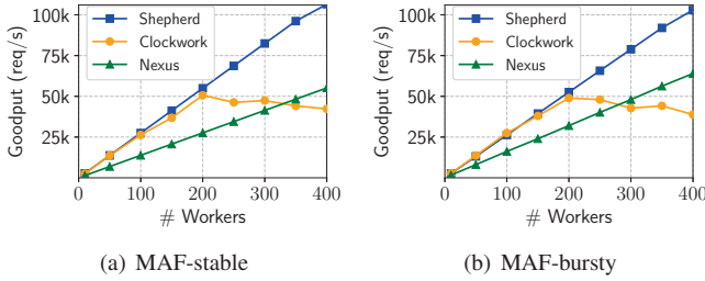
Figure 10: Scheduler scalability with emulated workers. For both workloads, Clockwork does not scale beyond 200 workers; Nexus scales linearly but observes 40–50% lower goodput than SHEPHERD. SHEPHERD observes both high goodput and linear scaling.
