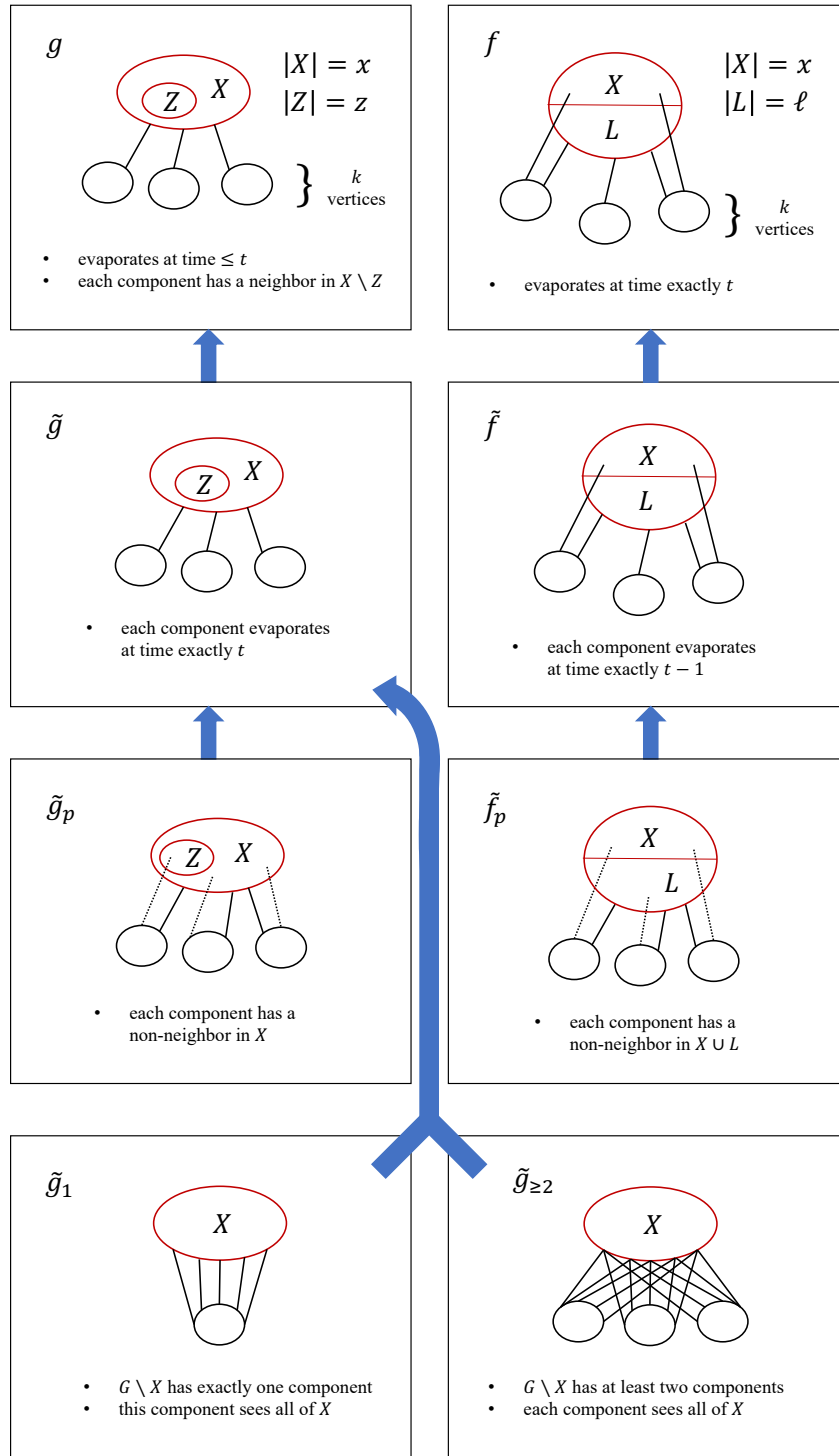
Figure 1 The counter functions. Here L = L_G(X) and Z = [z] . An arrow from one function to another, say from \tilde{g} to g , indicates that the definition of \tilde{g} is the same as that of g , except where indicated otherwise. The drawing of \tilde{f}_p represents \tilde{f}_p(t, x, \ell, k) . The function \tilde{f}_p(t, x, \ell, k, z) is similar but also keeps track of the argument z .
