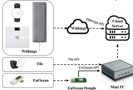
Figure 4: Data flow diagram in the sensor system.
