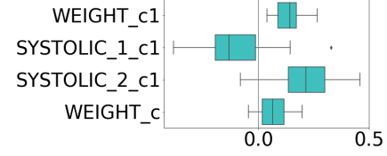
Figure 3: Variable coefficient variance.
