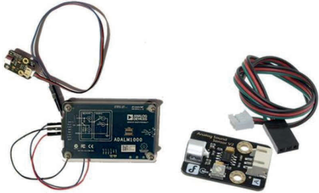
Figure 2: Sound Experiment Setup
