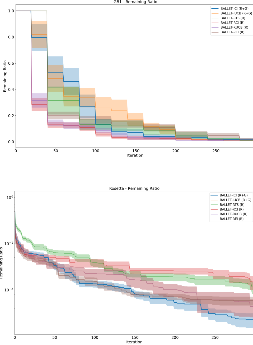
Figure 6: Simulation results on each task are shown here. The error bar demonstrates the standard error. The x-axis denotes the number of iterations, and the y-axis denotes the filtering ratio. The ratio for the 10 initial randomly picked warm-up datasets are clipped. (G), (R), and (R+G) means the global model only, the ROI model only, and the ROI model combined with the global model correspondingly.
