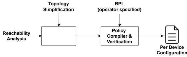
Figure 3: Aura architecture.
