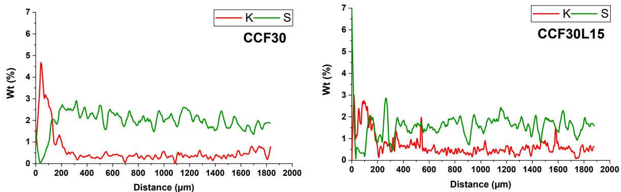
Figure 4 Line scan using EDX on showing difference in the distribution of sulphates and alkalis along the carbonation front
