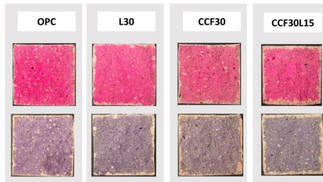
Figure 1 Carbonation measurement in cement mortar after 1 year of carbonation exposure (Atmospheric CO 2 and RH 57%) using 1% phenolphthalein and 1% thymolphthalein indicator
