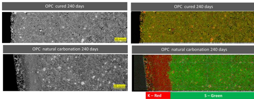
Figure 3 Microscopic image and elemental distribution of OPC sealed cured and carbonated for 240 days.
