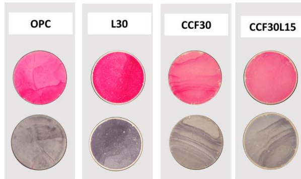
Figure 2 Carbonation measurement on cement after 240 days of carbonation exposure (Atmospheric \text{CO}_2 and RH 57%) using 1% phenolphthalein and 1% thymolphthalein indicator
