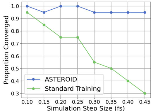
(b) Proportion of converged simulations (Aspirin).
