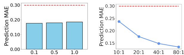
(a) Sensitivity study for \gamma (ethanol). The red line represents standard training.
