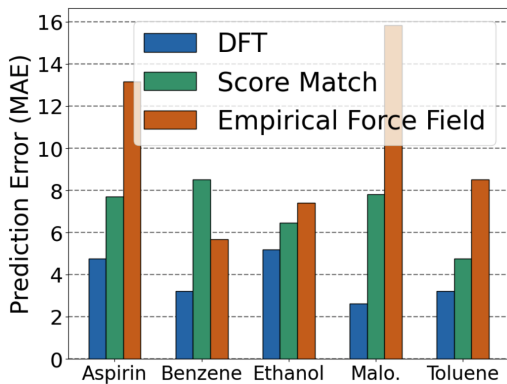
Figure 5. Prediction errors of models tested on CCSD(T) data. Models are not fine-tuned on the CCSD(T) data.
