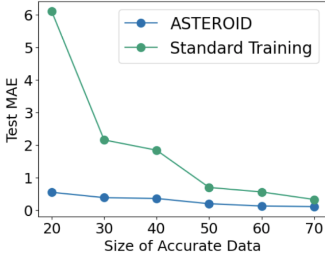
Figure 9. Asteroid toy example.
