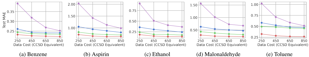
Figure 4. Main results for EGNN when DFT data is viewed as inaccurate. The legend is the same as in Figure 3.
