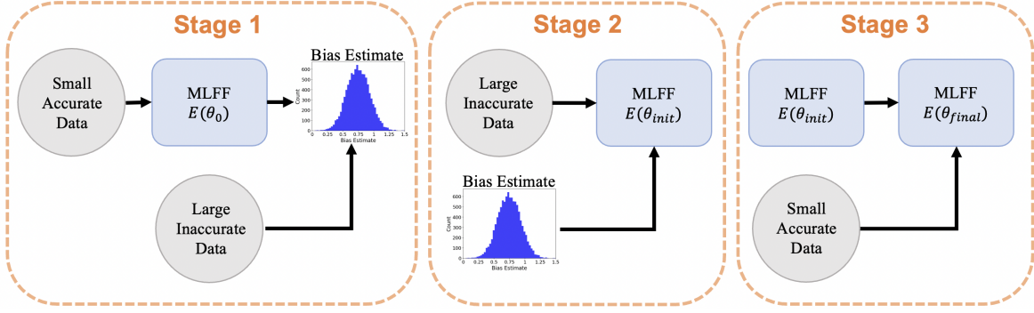
Figure 2. Asteroid workflow diagram. In stage 1, ASTERIOD uses the accurate data to estimate the bias in the inaccurate data. In stage 2, the MLFF is trained in a bias-aware manner on the inaccurate data. In stage 3, the MLFF is fine-tuned on the accurate data.
