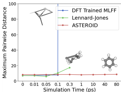
(a) Benzene molecule during MD simulation. Note that we use a non-linear time scale for clarity.
