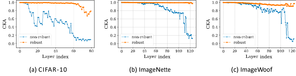
Figure 4: Divergence of adversarial representations from benign ones. We observe how adversarial perturbations, which are known to heavily impact model output, distort the internal representations in comparison to non-adversarial representations. We compare adversarial representations from corresponding layers in non-robust and robust networks. As expected, adversarial and benign representations in non-robust networks display high dissimilarity by the end of network. Unexpectedly, such divergence is very small for a non-trivial fraction of early layers (up to one-third). Robust training successfully reduces the impact of adversarial perturbations, thus leading to similar benign and adversarial representations in robust networks.
