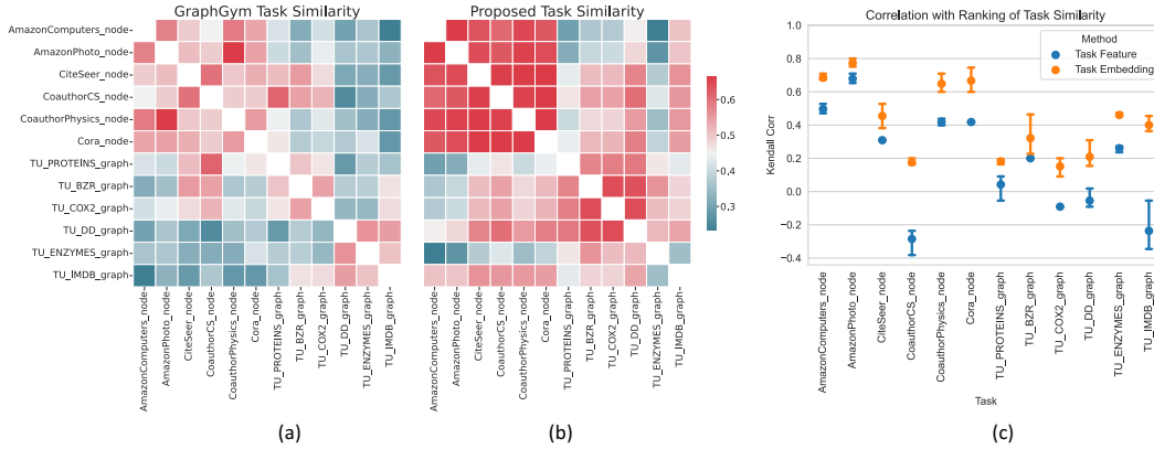
Figure 4: (a) GraphGym’s task similarity between all pairs of tasks (computed from the Kendall rank correlation between performance rankings of models trained on the two compared tasks), a higher value represents a higher similarity. (b) The proposed task similarity computed by computing the dot-product between extracted task features. (c) The Kendall rank correlation of similarity rankings of the other tasks with respect to the central task between the proposed method and GraphGym.
