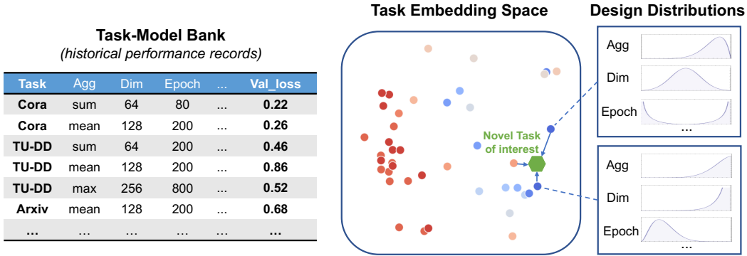
Figure 1: Overview of AUTOTRANSFER. Left: We introduce GNN-BANK-101, a large database containing a diverse set of GNN architectures and hyperparameters applied to different tasks, along with their training/evaluation statistics. Middle: We introduce a task embedding space , where each point corresponds to a different task. Tasks close in the embedding space have similar corresponding top-performing models. Right: Given a new task of interest, we guide the AutoML search by referencing the design distributions of the most similar tasks in the task embedding space.
