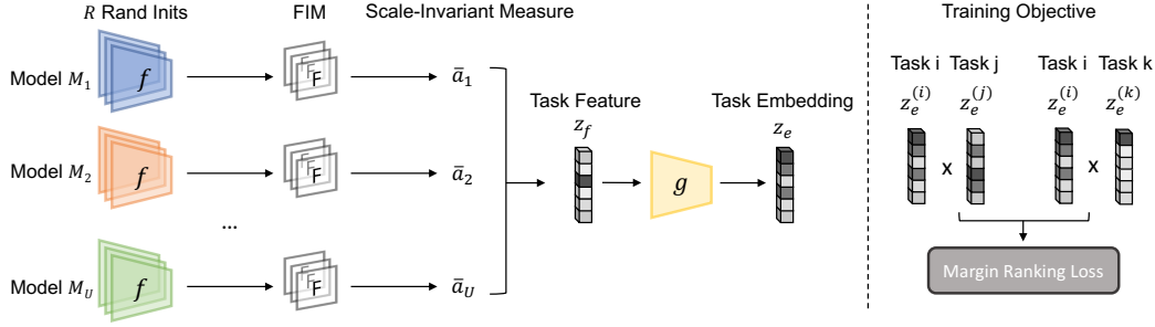
Figure 2: Pipeline for extracting task embeddings. Left: To efficiently embed a task, we first extract task features by concatenating features measured from R randomly initialized anchor models. Then, we introduce a projection function g(\cdot) with learned weights to transform the task features into task embeddings. Right: Training objective for optimizing g(\cdot) with triplet supervision.
