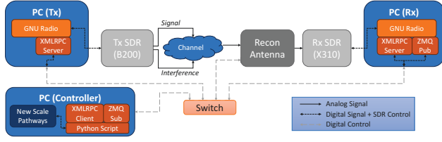
Figure 5. Testbed architecture and software configuration
