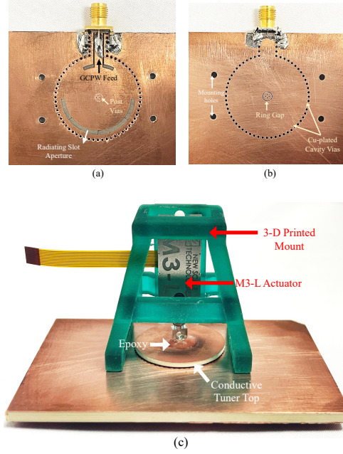
Figure 2. Fabricated Prototype of the tunable antenna (a) Bottom-view with the feed and radiating slot aperture (b) Top-View (c) Full assembly with the M3-L linear actuator and the 3-D printed mount.
