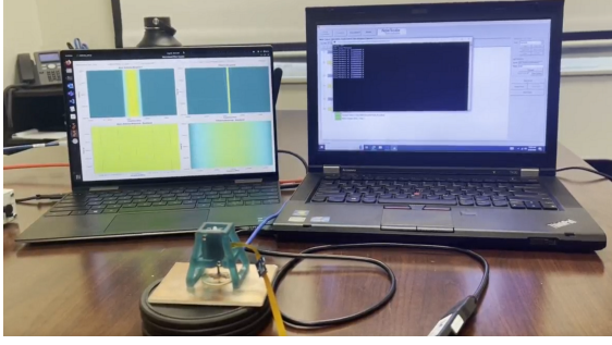
Figure 9. Physical deployment demonstrating control node (Windows PC, right) with New Scale Pathway software, the tunable antenna, and receive node (Linux PC, left) running GNURadio.
