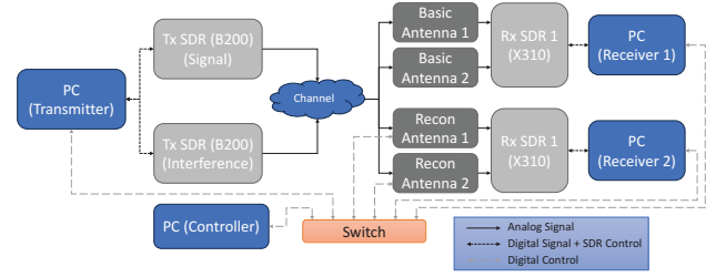
Figure 6. Extended Testbed Architecture (future)
