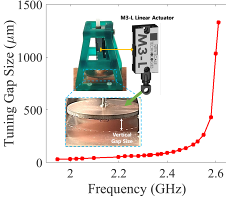
Figure 3. Measured tuning curve for the reconfigurable antenna. The center frequency of the antenna is tuned by vertically placing the conductive disk across a large range of gap sizes.
