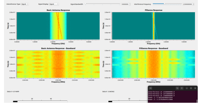
Figure 8. Simulation results showing automated configuration of signal and interference parameters via XMLRPC and power measurements via ZMQ (configured from Python script on the GNU-Radio computer via localhost connections).
