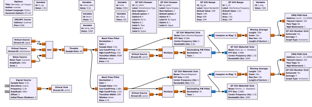
Figure 7. Multi-rate flowgraph to simulate basic and tunable antenna responses and demonstrate out-of-band interference that is introduced without proper filtering prior to down-conversion.
