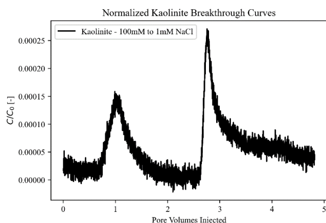
Fig. 2. Normalized breakthrough curve of 150mM kaolinite suspended in 100mM NaCl injected into Ottawa sand column that had been saturated with a 100mM NaCl solution (pH=7). Injection fluid salinity was changed to 1mM NaCl when pore volumes injected was 2.17 (40 minutes).
