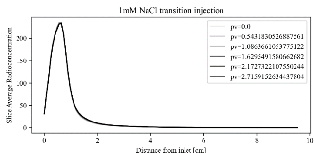
Fig. 6. Transition from 64 Cu 2+ radiolabeled kaolinite in 100mM NaCl solution to a 1mM NaCl solution saturating the homogenous Ottawa sand pack column as a function of column length. This plot shows the transition from higher to lower ionic strength, so pore volume 0 is seen on the top of the plot of the plot since radiolabeled kaolinite was in the column when the PET scan began. Breakthrough is plotted as a summation of slice averaged radioconcentration as a function of pore volumes injected.
