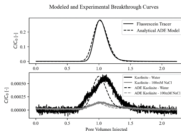
Fig. 3. Top) Normalized experimental tracer from column experiment (solid black) and the analytically modelled tracer (dashed black) from the ADE with reaction solution from Parker and van Genuchten [22]. Bottom) Normalized breakthrough curves of 150mM kaolinite suspended in DI water injected into Ottawa sand column that had been saturated with DI water (black curve with higher peak), analytically derived breakthrough curve (dashed black), 150mM kaolinite suspended in 100mM NaCl injected into Ottawa sand column that had been saturated with 100mM NaCl (grey curve with lower peak), and analytically derived breakthrough curve (dashed grey).
