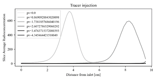
Fig. 4. Normalized [ 18 F]FDG tracer pulse concentration profiles through a homogenous Ottawa sand pack as a function of column length. Breakthrough is plotted as a summation of slice averaged radioconcentration as a function of pore volumes injected.
