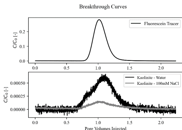
Fig. 1. Top) Normalized breakthrough curve of conservative fluorescein injected into Ottawa sand column that had been saturated with DI water. Bottom) Normalized breakthrough curves of 150mM kaolinite suspended in DI water injected into Ottawa sand column that had been saturated with DI water (black curve with higher peak) and 150mM kaolinite suspended in 100mM NaCl injected into Ottawa sand column that had been saturated with 100mM NaCl (grey curve with lower peak). The pH of all solutions is at a pH of 7. Both plots are plotted as a function of pore volumes injected.
