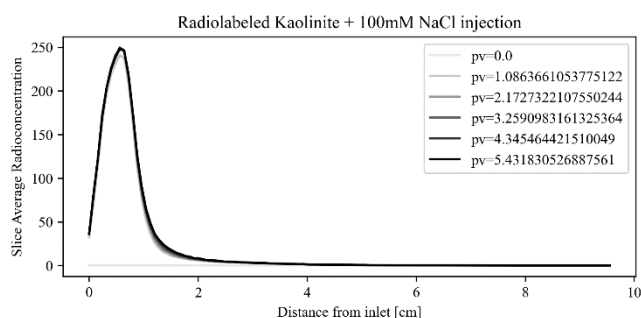
Fig. 5. Normalized 64 Cu 2+ radiolabeled kaolinite in 100mM NaCl concentration profiles through a homogenous Ottawa sand pack as a function of column length. This plot shows the injection of kaolinite into the sand pack. Pore volume 0 is seen on the bottom of the plot since no radioisotope has been imaged yet. Breakthrough is plotted as a summation of slice averaged radioconcentration as a function of pore volumes injected.
