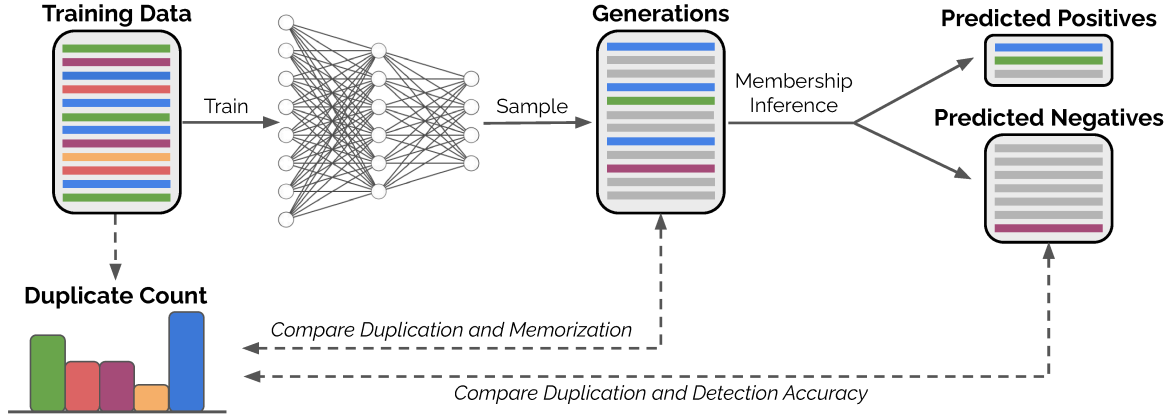
Figure 2. Overview of our analysis. Web-scraped text datasets that are used to train language models contain duplicated sequences, depicted in the figure as training data rows of the same color (top left). Model inversion attacks attempt to recover training data from a trained model by first generating large amounts of text, some of which is memorized training data (top middle). Membership inference is then performed to detect which generated sequences were copied from the training data (top right). Our analysis focuses on the relationship between the amount a sequence is duplicated in the training data and the effectiveness of the model inversion attack at generating and detecting that sequence (bottom).
