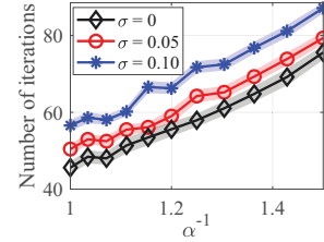
Figure 5: The number of iterations against \alpha
