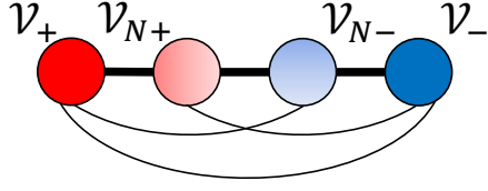
Figure 22: Toy example of the data model. Node 1 and 2 have label +1 . Nodes 3 and 4 are labeled as -1 . Nodes 1 and 4 have class-relevant features. Nodes 2 and 3 have class-irrelevant features. \mathcal{V}_+ = \{1\} , \mathcal{V}_{N+} = \{2\} , \mathcal{V}_{N-} = \{3\} , \mathcal{V}_- = \{4\} .
