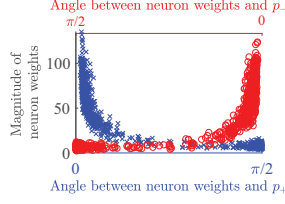
Figure 7: Distribution of the neuron weights
