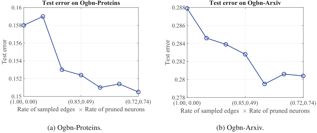
Figure 27: Test error on (a) Ogbn-Proteins and (b) Ogbn-Arxiv.
