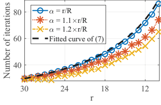
Figure 16: Number of iterations against the edge sampling rate with random &amp; important sampling.
