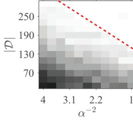
Figure 3: |\mathcal{D}| against the importance sampling probability \alpha
