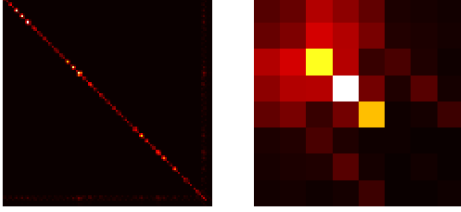
Fig. 3: A comparison of the structure of the Dong-Si [20] A^T A (left) and the proposed A'^T A' (right). The Dong-Si system contains 35 features here (making it 111 \times 111 ). While sparse, it is much larger than ours, which is 8 \times 8 no matter how many features are included. The log condition number for Dong-Si's is 9.35 while the proposed is 8.15.
