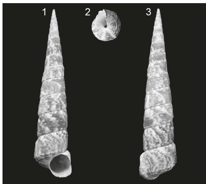
Text-fig. 12. Caviturritella gonostoma (Valenciennes, 1832), the type species designated for Caviturritella Friend and Anderson, new genus. Specimen PRI 104787 is from an unspecified locality but extant Caviturritella gonostoma are found in the eastern Pacific from the Gulf of California to Peru. Specimen length 116.6 mm.
