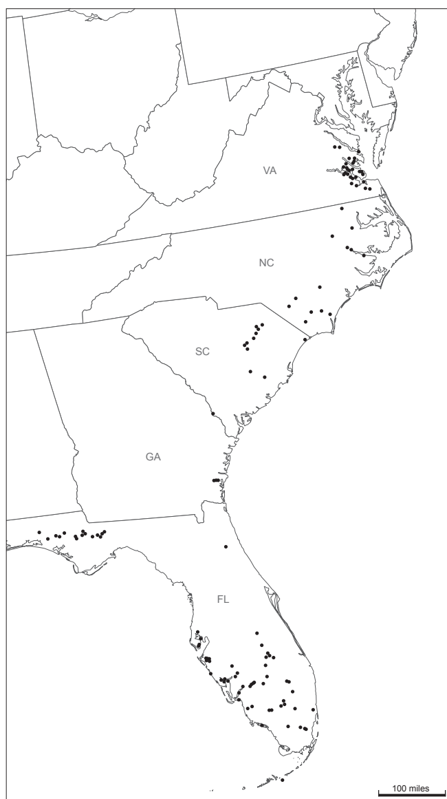
Text-fig. 2. Geographic distribution of localities referenced in the present manuscript. For a complete list of locality information see Appendix 1.
