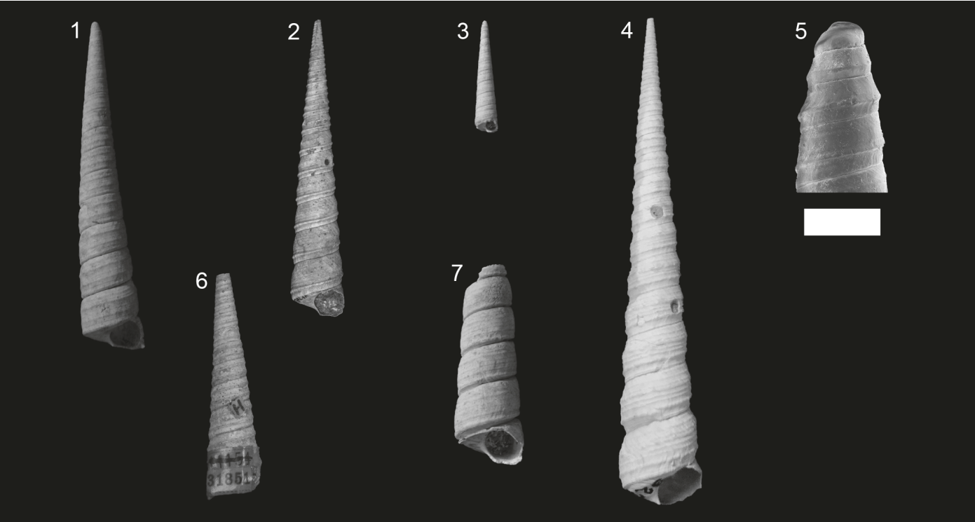
Text-fig. 15. Caviturritella etiwanensis (Tuomey and Holmes, 1856). 1, PRI 104826, NC-07, 52.5 mm. 2, UF 7683, FL-68, 40.4 mm. 3, PRI 104828, NC-07, 17.3 mm. 4, USNM 370331, FL-19, 103.5 mm. 5, protoconch, PRI 104737, NC-10, scale bar = 1 mm. 6, lectotype, AMNH FI 31851, SC-13. 7, PRI 104827 from NC-07, 37.6 mm.
