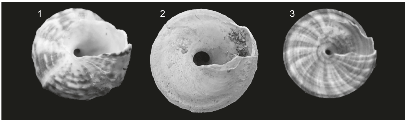
Text-fig. 11. Turritellids with hollow newels. These species lack a columella and instead have cavities visible from the basal surface that opens into the body chamber, facilitating access to the body chamber of more apical whorls than the apertural whorl (e.g., when probed with a pin). 1, Caviturritella gonostoma , PRI 104787, Recent, tropical eastern Pacific, diameter 27.5 mm. 2, Caviturritella alumensis , PRI 41858, FL-02, diameter 24.1 mm. 3, Caviturritella magnasulcus , UF 332525, FL-80, diameter 9.2 mm.
