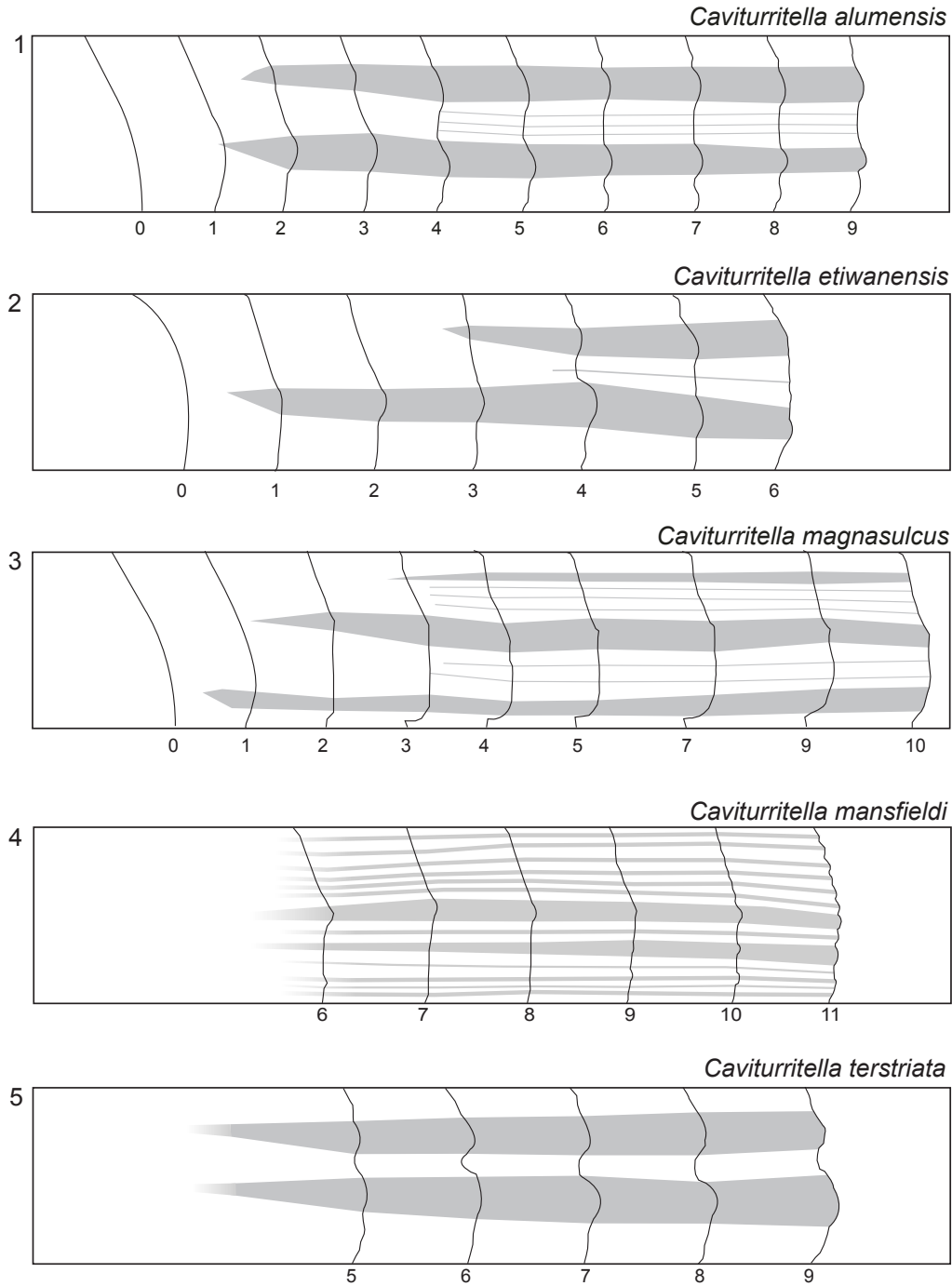
Text-fig. 6. Marwick diagrams depicting the ontogenetic development of spiral cords in Caviturritella Friend and Anderson, n. gen. (herein). Numbers at the bottom represent whorl number, the protoconch and youngest whorls being on the left. All whorl outlines are standardized to the same height. Note that Caviturritella alumensis cord A does not appear until ~whorl 14 (not shown). We lack protoconchs of C. terstriata and C. mansfieldi and so therefore the beginning whorl numbers are approximations. See pp. 7, 8 for more information on these schematic diagrams.
