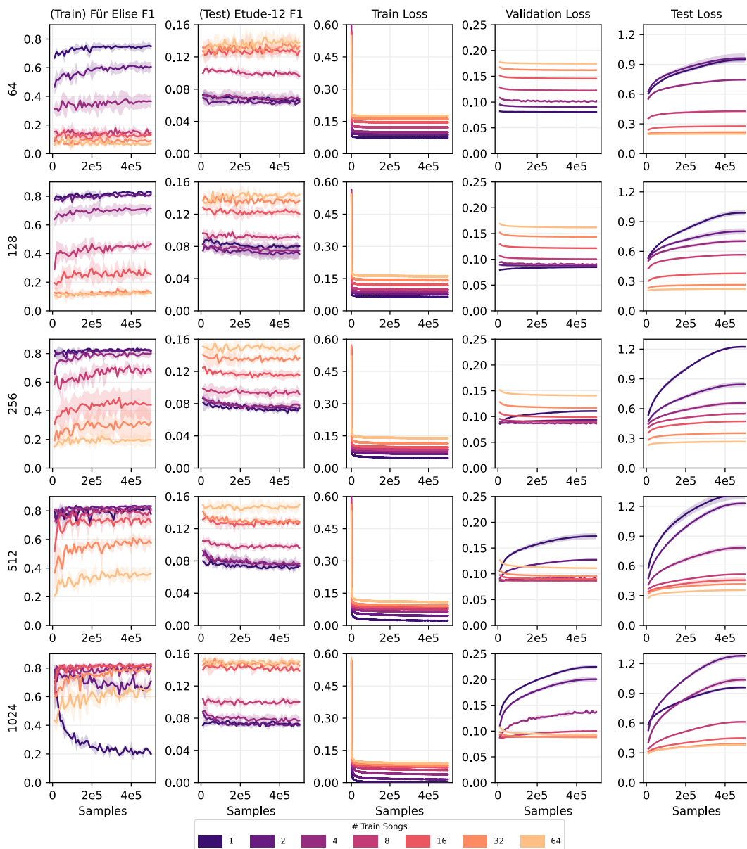
Figure 10: Detailed multi-task BC results.
