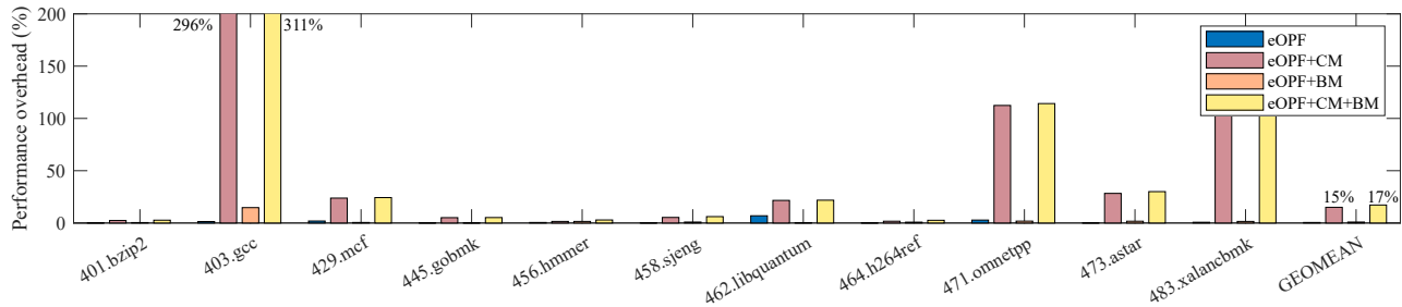
Figure 8: SPEC CPU 2006 performance with eOPF using the reference dataset on the server machine. The enclave partition was 1/12 \times \text{LLC} . For this test, the enclave exits per-second were: 3, 105, 4, 3, 3, 2, 2, 1, 11, 1, 8, from left to right.
