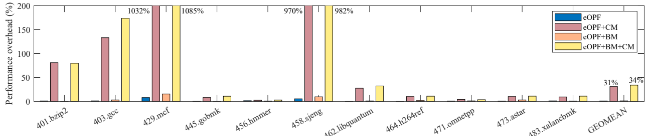
Figure 9: SPEC CPU 2006 performance with eOPF using the test dataset on the desktop machine. The enclave partition was 1/8 \times \text{LLC} . For this test, the enclave exits per-second were 29, 2184, 3071, 965, 25, 3444, 417, 298, 60, 22, 91, from left to right.
