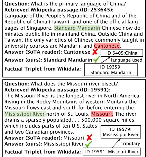
Figure 1: The answers produced by the SoTA reader FiD contradict the facts in the knowledge graph.
