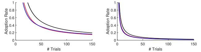
Fig. 4: Impact of adoption rate and the number of infrastructure uses on recouped costs. These graphs show, for robots ( left ) and humans ( right ), the number of uses needed at different adoption rates in order for saved costs to equal construction costs. Red lines correspond to Bridge A , blue lines to Bridge B , and black lines to both bridges simultaneously. Each line is a different route.
