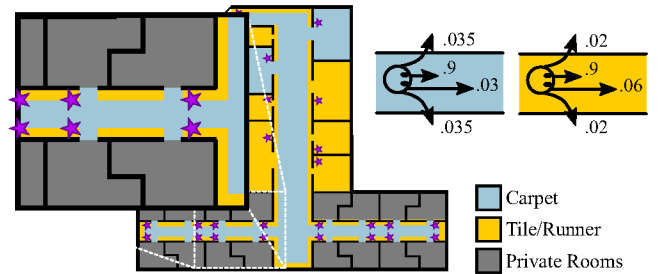
Fig. 1: An example long-term care facility. Purple stars are potential goals. The robot takes 5s to travel 1m on carpet, and 3s to travel 1m on tile. Transition probabilities for the floors are shown.
