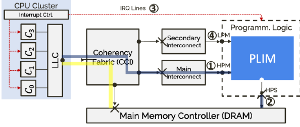
Figure 3: PLIM module instantiation on a PS-PL platform.
