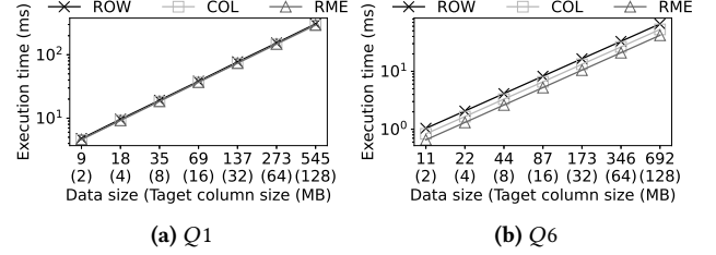
Figure 13: RME scales with data size and shows stable performance in practical queries such as TPC-H Q_1 and Q_6 .
