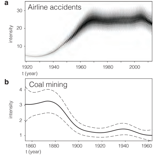
Figure 15: a) Mean airline accidents intensity and the 95% credible interval. b) Mean coal mining explosion accidents and 95% credible interval.
