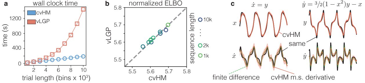
Figure 2: (a) cvHM inference scales better than vLGP. Sequence length varies from 1k to 10k in intervals of 1k. Hyperparameters of both methods are kept constant. (b) Normalized ELBO (nats/bin) comparison shows same quality inference. (c) Van der Pol oscillator experiment. (top) cvHM inference on the 2D latents. (bottom) Time derivative of x and y , and corresponding mean square derivatives inferred by cvHM compared to finite difference of the inferred mean; GP inferred derivatives come at no additional cost and offer calibrated measure of uncertainty that may be useful in latent trajectory analysis to better understand neural computation.
