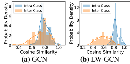
Figure 4: Representation similarity distributions on Texas Graphs.
