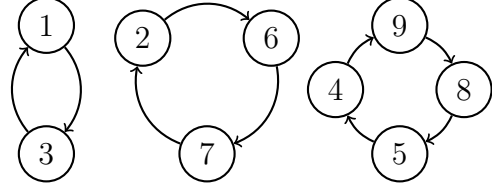
Figure 18: The associated G(s) .
