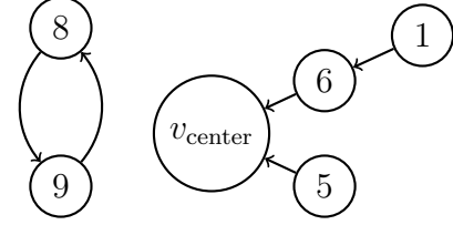
Figure 4: The associated G(t) .
