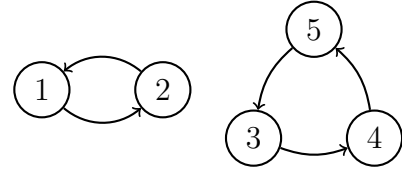
Figure 10: The associated G(t_{\text{cycles}}) .
