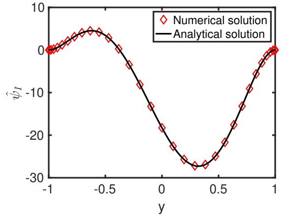
(b) Imaginary part, \hat{\psi}_I(y, t=5)
