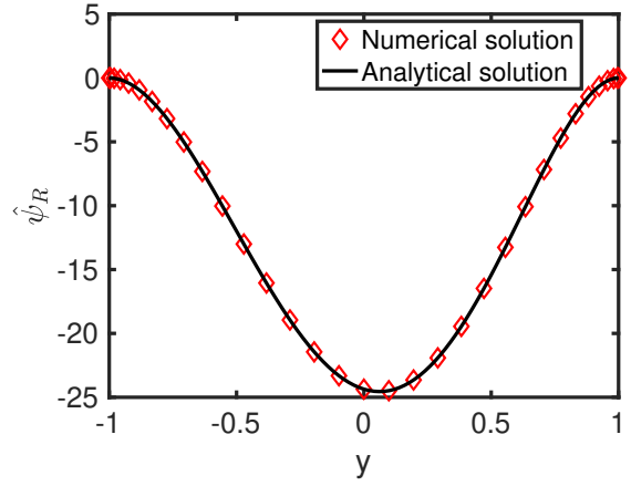
(a) Real part, \hat{\psi}_R(y, t=5)
