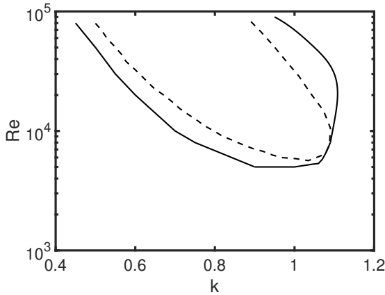
Fig. 2: Stability of 2D LNS equation via LPIs (solid line) compared to an eigenvalue stability for a plane Poiseuille flow (dashed line). Unstable regions are inside the curves. Plot is in agreement with Corollary 1 : S_{Lyap}(k, Re) \subseteq S_{eig}(k, Re) .
