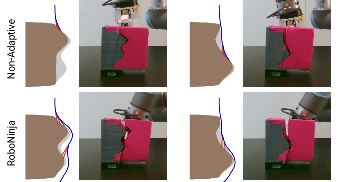
Fig. 12: Real-world comparison. [Non-Adaptive] has the drawback of getting stuck even when the state estimation is very close. In contrast, [RoboNinja] leverages an adaptive cutting policy that allows it to bypass the peak and successfully reach the bottom.
