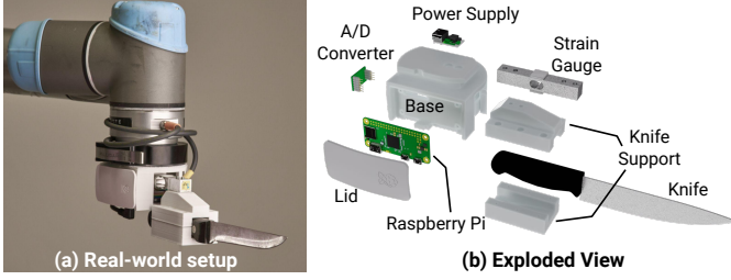
Fig. 5: Hardware. We design and construct a compact cutting tool equipped with a force sensor. The force is measured by a strain gauge as an analog electrical signal. The signal is then converted to a digital signal and transmitted to the robot controller through an A/D converter and a Raspberry Pi Zero, respectively.
