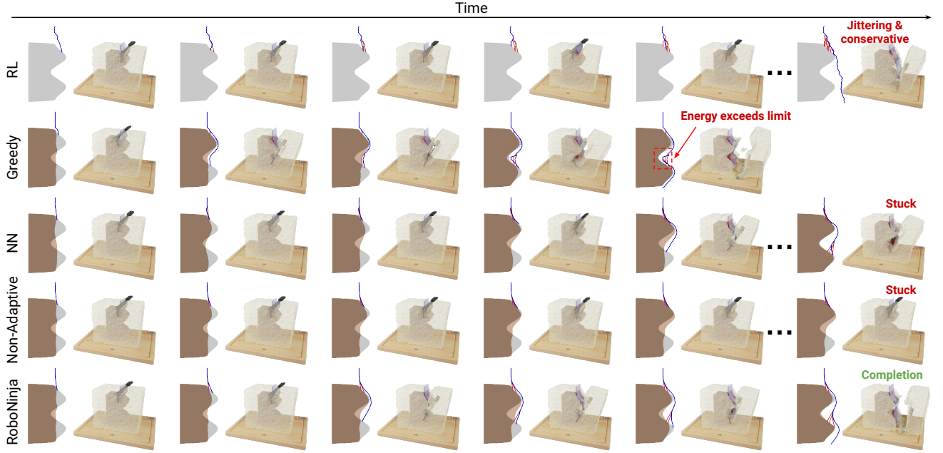
Fig. 8: Evaluation on in-distribution geometries. Each column shows an iteration (continuous execution until a collision). In the 2D view (left), the ground truth geometry is shown in gray, and the estimation is shown in brown. In both views, the forward trajectory of the knife is demonstrated in blue, and the retraction trajectories due to collision are visualized in red. The cutting trajectory of [RL] is very jittering and becomes too conservative after a few collisions. [Greedy] strictly follows the contour of the estimated geometry, leading to exceeding energy consumption during abrupt rotations. Both [NN] and [Non-Adaptive] can’t complete the cutting task within 10 collisions. [RoboNinja] is able to iteratively update the estimate of the core after each collision and adaptively adjust the cutting trajectory with optimized energy consumption.
