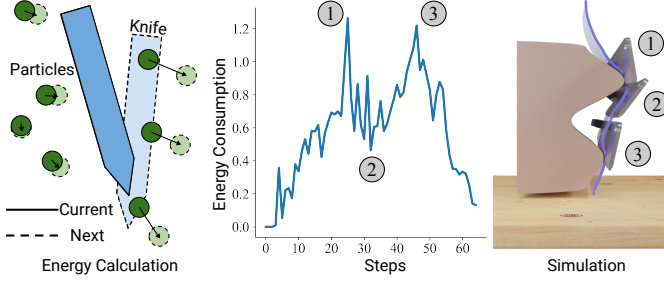
Fig. 3: Energy Calculation. [Left] Illustration of energy computation in simulation. Particle position and velocity are changed due to collision with the knife. The cumulative work from the knife to each collided particle is considered as the energy consumption of the agent. [Middle] A plot of energy consumption at each step. [Right] Visualization of knife poses at some representative steps. Note that large energy consumption incurs around the rapid rotations in the trajectory. (e.g., steps 1 and 3).
