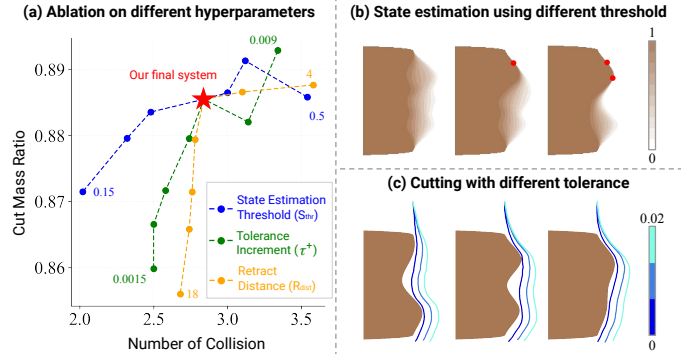
Fig. 11: Ablations on algorithm parameters. [Left] summarizes the effects of several critical hyperparameters in the algorithm. Detailed discussion about their effects and trade-off can be found in Sec. IV-C. [Right-Up] State estimation results with different thresholds. [Right-Bottom] Cutting trajectories with different tolerance increments.
