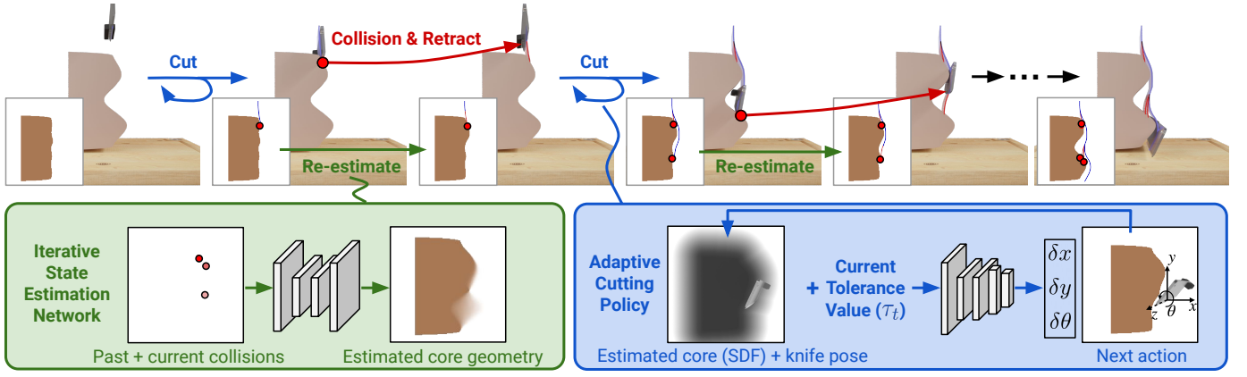
Fig. 2: RoboNinja Overview. The robot initially performs actions based on an initial estimation. In the event of a collision with the rigid core, the robot retracts a few steps (indicated in red). The robot then re-estimates the core’s position and geometry (indicated in green) and generates the cutting action using the updated state estimation (indicated in blue).
