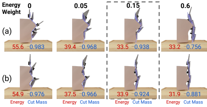
Fig. 10: Trajectories optimized with different weights of energy loss. Cumulative energy consumption and the cut mass ratio are shown in red and blue, respectively. Without any energy penalty, the trajectory strictly follows the contour of the core and cuts off most of the soft material. However, the knife has to rotate rapidly to avoid collision with the core, which results in large energy consumption. In contrast, a large energy penalty leads to a conservative policy where the rotation of the knife is less noticeable. An appropriate energy weight achieves a balance between energy consumption and cut mass. The one used in our final system [0.15] is able to cut off over 90% with similar energy consumption as [0.6].
