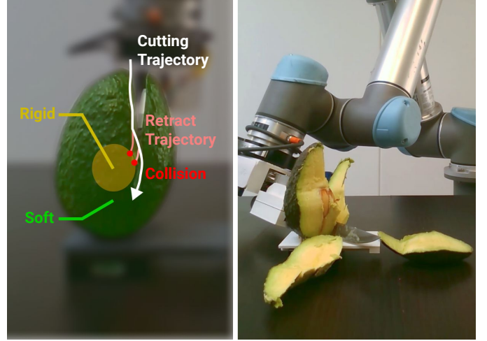
Fig. 1: RoboNinja is designed to cut multi-material objects with an interactive state estimator and adaptive cutting policy. Left: When the knife encounters a collision with the invisible core, the algorithm updates the core estimation and re-plans the cutting trajectory after a few retracting actions. Right: We deploy the learned model on a physical robot, allowing it to cut fruits in a way that maximizes the cut-off mass while minimizing collision occurrences.
