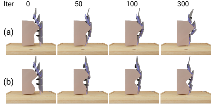
Fig. 4: Optimization Process of Cutting Trajectory. As illustrated in the first column, the cutting trajectory is initialized with a pre-designed collision-free path. After 300 optimization iterations, the knife is able to cut off most of the soft materials with optimized energy consumption.
