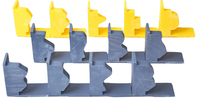
Fig. 7: 3D printed cores in real-world evaluation. 8 in-distribution geometries (gray) and 5 out-of-distribution geometries (yellow).
