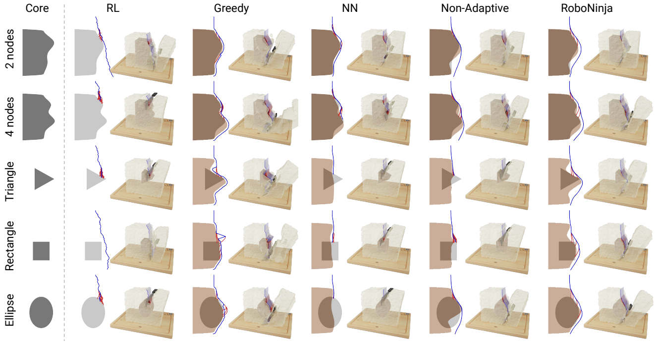
Fig. 9: Evaluation on out-of-distribution geometries. The cores sampled from each category are shown in the first column, followed by trajectories produced by each method. Both [NN] and [Non-Adaptive] may get stuck, especially when the geometries (e.g., Triangle and Rectangle) are significantly different from the training set. Both [Greedy] and [RoboNinja] have a strong generalization ability to handle various novel geometries. However, [RoboNinja] consumes much less energy than [Greedy], leading to smoother and more natural cutting trajectories.
