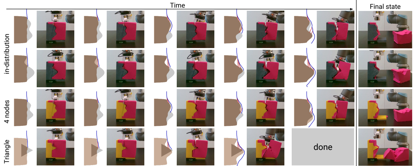
Fig. 14: Realworld evaluation on 3d printed cores and kinetic sand. Our simulation-trained policy demonstrates strong generalization capabilities, effectively handling both in-distribution and out-of-distribution cores in a real-world setting. With only a few collisions, it is able to accurately estimate the core geometry and cut off the majority of the sand with a smooth cutting trajectory.
