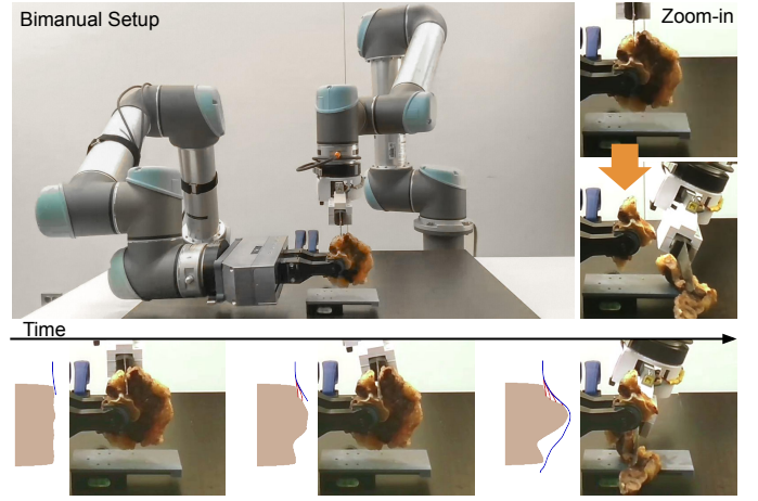
Fig. 15: Evaluation on real meat. We deploy our cutting policy on a bimanual setup, with one arm using a parallel-jaw gripper to hold the bone and the other arm using a knife to cut the meat. The cutting trajectory and core estimation are shown at the bottom.
