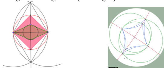
Figure 1. Quasi-Squares from rhombus as equilateral quadrilaterals with congruent diagonals extensible to Hyperbolic and Spherical Geometries
