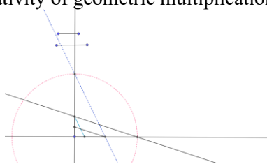
Figure 2. Geometric multiplication of given two segments
