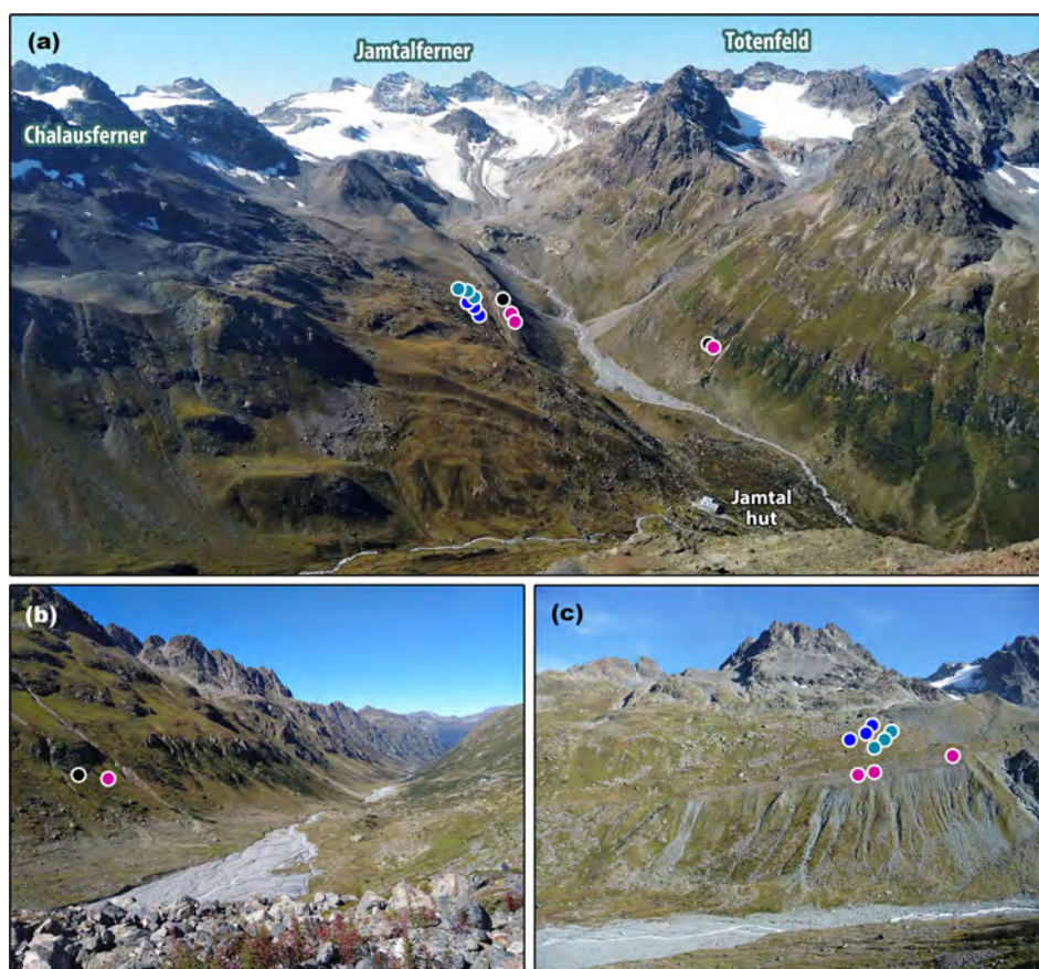
Figure 3. Photographs of Jamtal. (a) View toward Jamtalferner and Totenfeld. ^{10}\text{Be} sample locations are marked with colored circles (pink represents LIA; black represents Neoglacial, cyan and blue represent EH). (b) Down-valley view depicting sample locations JAM-18-06 (pink) and JAM-18-07 (black). (c) Valley flank below Chalausferner and Augustenferner with sampled boulders along the innermost (pink), middle (cyan), and outer (blue) right lateral moraine of former Chalausferner. For the broader context of the individual sites, see Fig. 1c.
