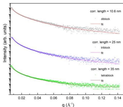
Figure 4 The log intensity vs. scattering vector ( q ) plots of the PLO-PLA diblock, triblock, and tetrablock copolymers.
