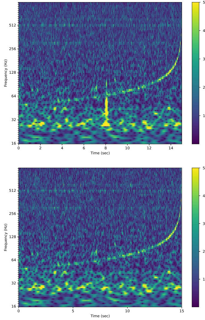
Figure 6. Subtraction of the Tomte Glitch. The top and bottom panels show the CQT of the data and residual, respectively. The glitch is the vertical feature at \approx 8.0 sec. In order to show both the glitch and the signal in the same image, a threshold has been applied to the CQT as indicated by the maximum value in the colorbar of the top panel.
