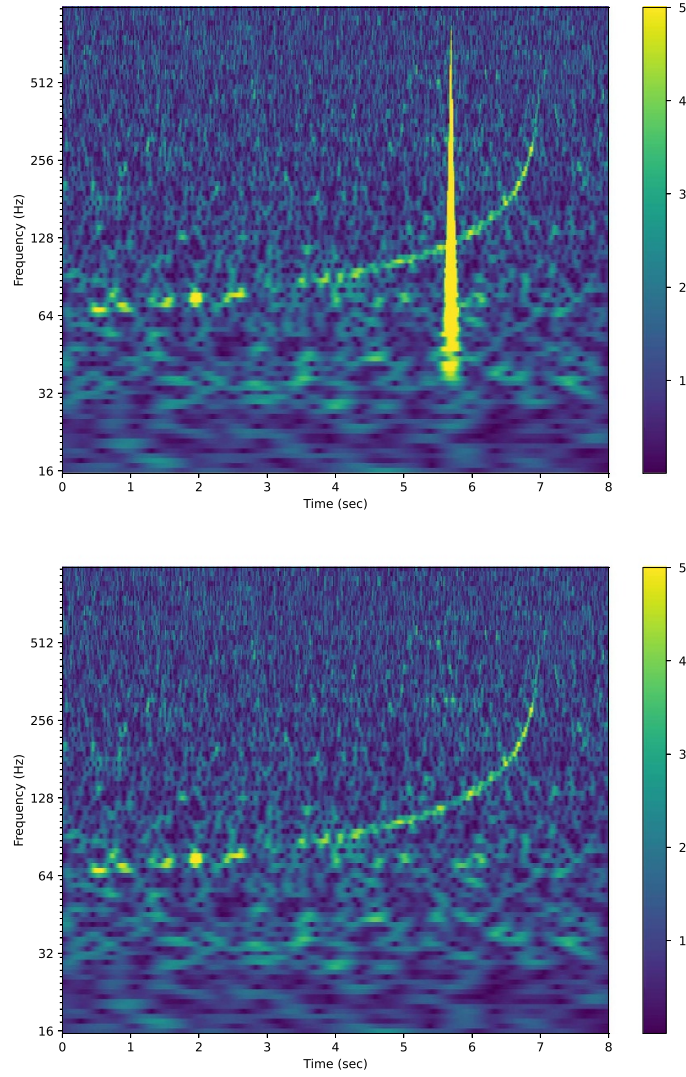
Figure 4. Subtraction of the Blip Glitch. The top and bottom panels show the CQT of the data and residual, respectively. The glitch is the vertical feature at \approx 6 sec. In order to show both the glitch and the signal in the same image, a threshold has been applied to the CQT as indicated by the maximum value in the colorbar of the top panel.
