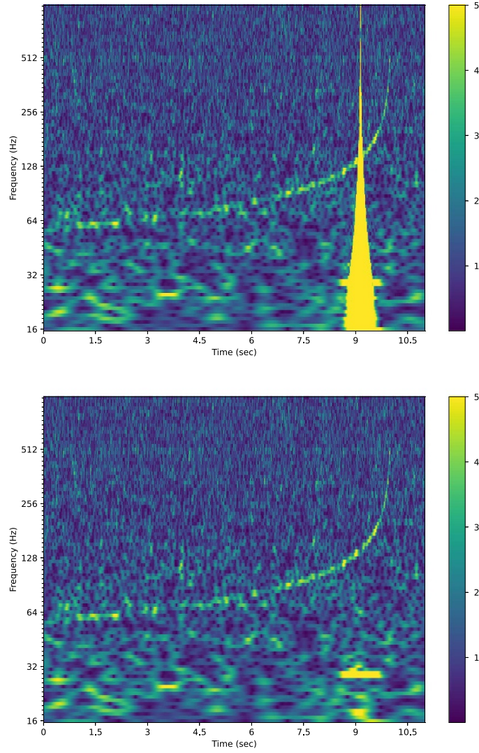
Figure 5. Subtraction of the Koi Fish glitch. The top and bottom panels show the CQT of the data and residual, respectively. The glitch is the vertical feature at \approx 9.0 sec. In order to show both the glitch and the signal in the same image, a threshold has been applied to the CQT as indicated by the maximum value in the colorbar of the top panel.
