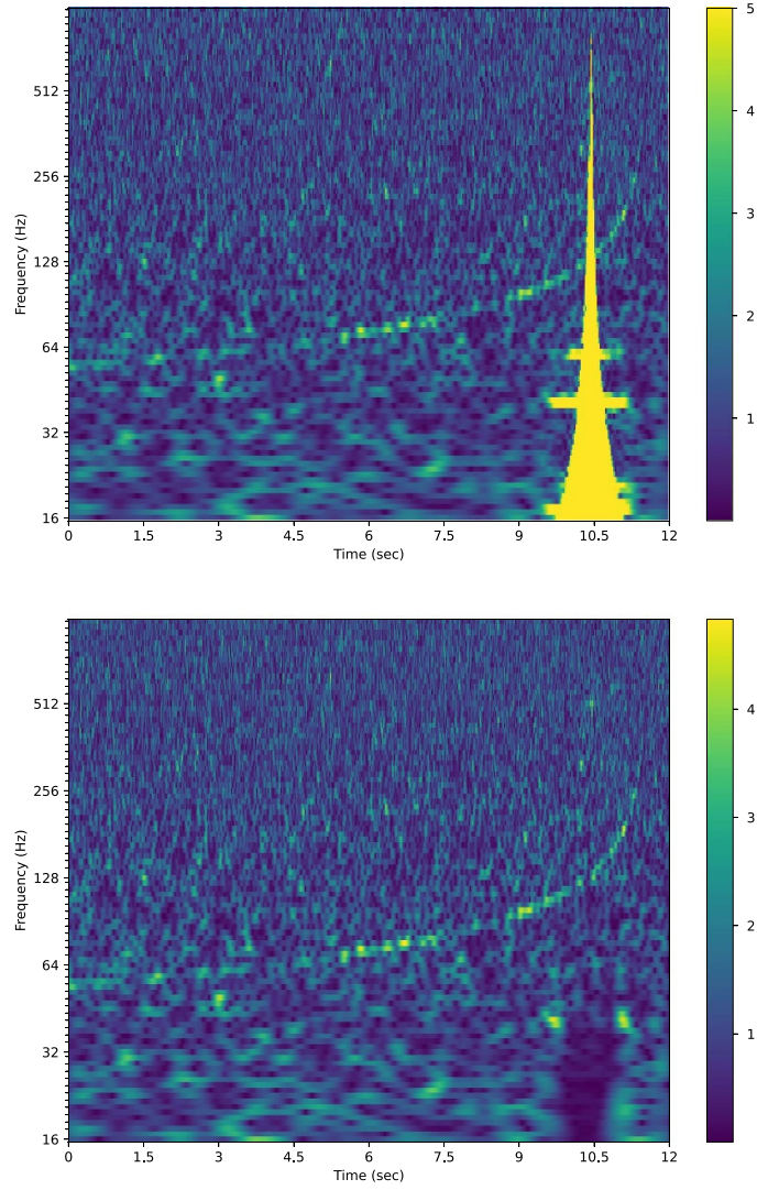
Figure 3. Subtraction of the GW170817 Glitch. The top and bottom panels show the CQT of the data and residual, respectively. The glitch is the vertical feature at \approx 10.5 sec. In order to show both the glitch and the signal in the same image, a threshold has been applied to the CQT as indicated by the maximum value in the colorbar of the top panel.
