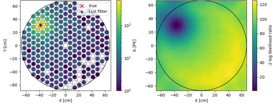
Figure 3: (Left) An example of reconstructed position using a likelihood fitter built with the trained MLP model. The smaller circles represent the photosensors and the color marks k_i for each photo-sensor. (Right) The result of a likelihood scan using the trained MLP model. The black circle marks the boundary of the considered LXeTPC detector.
