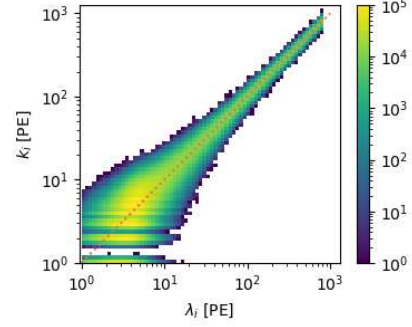
Figure 1: A comparison of expectation value of the signal \lambda_i and simulated observed value k_i in the synthetic data set.
