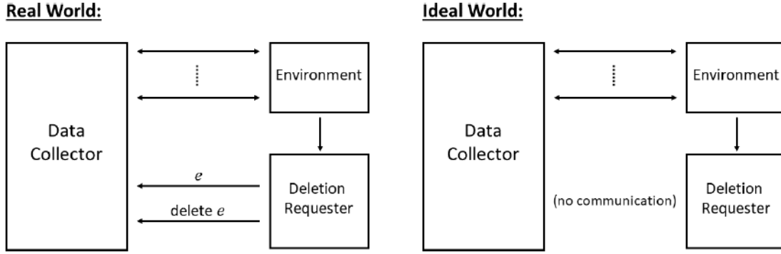
Fig. 4. The real and ideal worlds for (strong) deletion compliance
