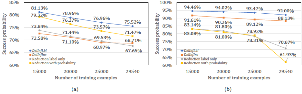
Fig. 1. Trend of success probabilities of attacks Del-Inf-Exm and Del-Inf-Ins on smallCNN models trained with different number of examples are shown; (a) uses dataset CIFAR-10 and (b) uses dataset CIFAR-100 dataset. The success probabilities are also compared with two baseline attacks that are obtained by reductions to the membership inference attack of [SSSS17].
