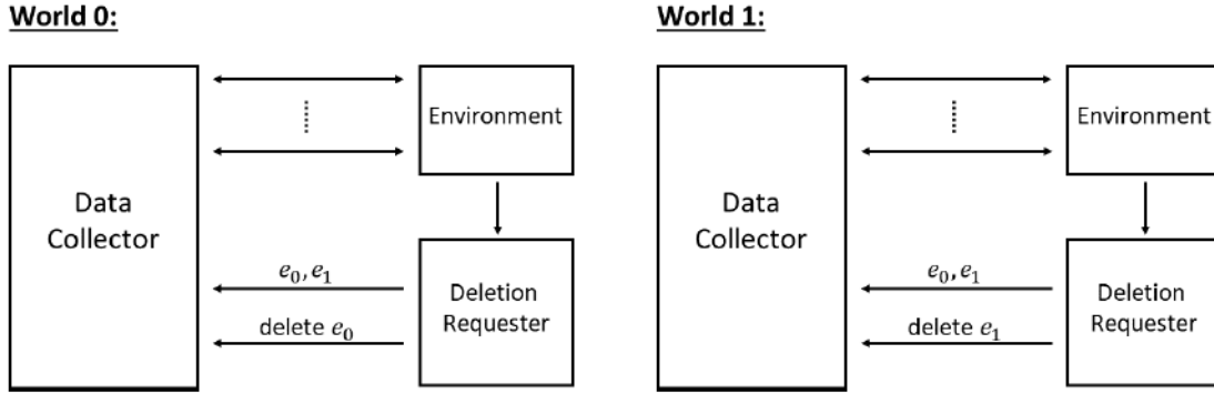
Fig. 5. The worlds for weak deletion-compliance
